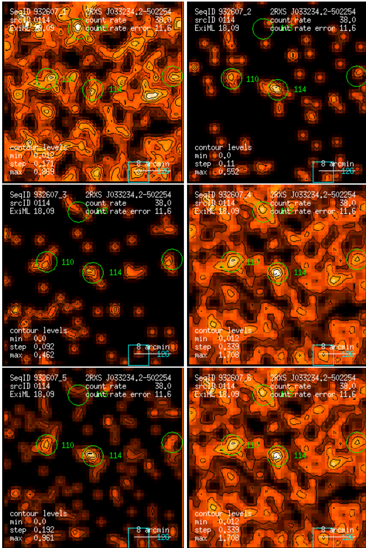
Figure 114: RASS 932607: detection 0114: band rate images, Gaussian filter: (1) PSPC channels 11 – 41, (2) 52 – 90, (3) 91 – 201, (4) 11 – 235, (5) 52 – 201, (6) 11 – 201. Broad band rates in counts/ks. Band rate contour levels in counts/ks/arcmin 2 .
