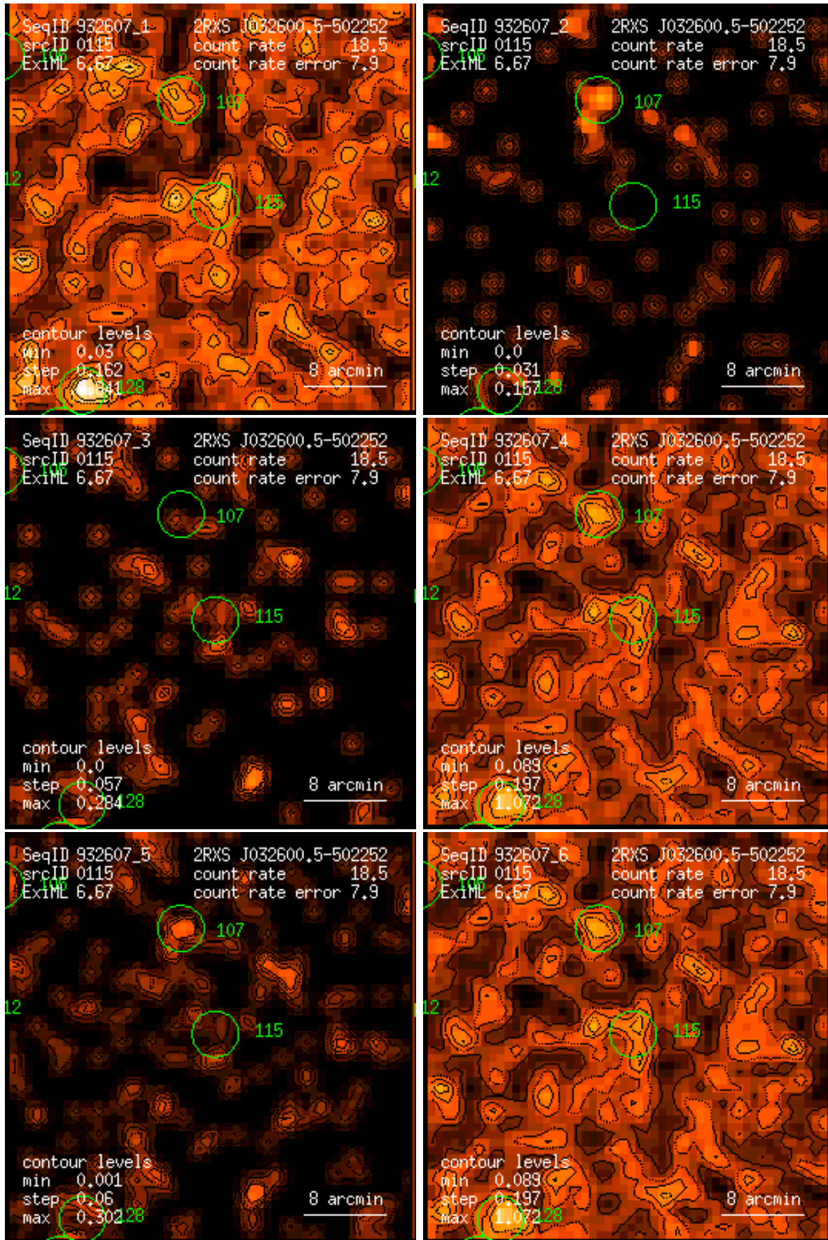
Figure 115: RASS 932607: detection 0115: band rate images, Gaussian filter: (1) PSPC channels 11 – 41, (2) 52 – 90, (3) 91 – 201, (4) 11 – 235, (5) 52 – 201, (6) 11 – 201. Broad band rates in counts/ks. Band rate contour levels in counts/ks/arcmin 2 .
