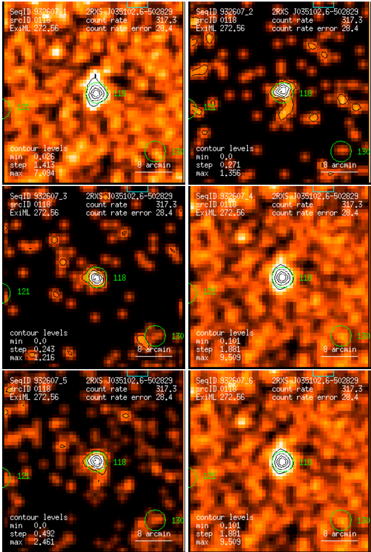
Figure 118: RASS 932607: detection 0118: band rate images, Gaussian filter: (1) PSPC channels 11 – 41, (2) 52 – 90, (3) 91 – 201, (4) 11 – 235, (5) 52 – 201, (6) 11 – 201. Broad band rates in counts/ks. Band rate contour levels in counts/ks/arcmin 2 .
