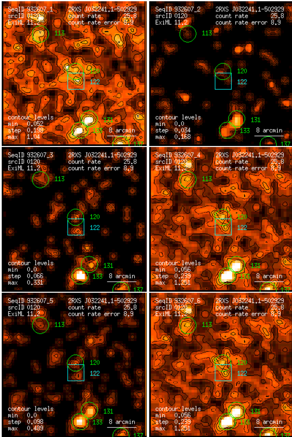
Figure 120: RASS 932607: detection 0120: band rate images, Gaussian filter: (1) PSPC channels 11 – 41, (2) 52 – 90, (3) 91 – 201, (4) 11 – 235, (5) 52 – 201, (6) 11 – 201. Broad band rates in counts/ks. Band rate contour levels in counts/ks/arcmin 2 .
