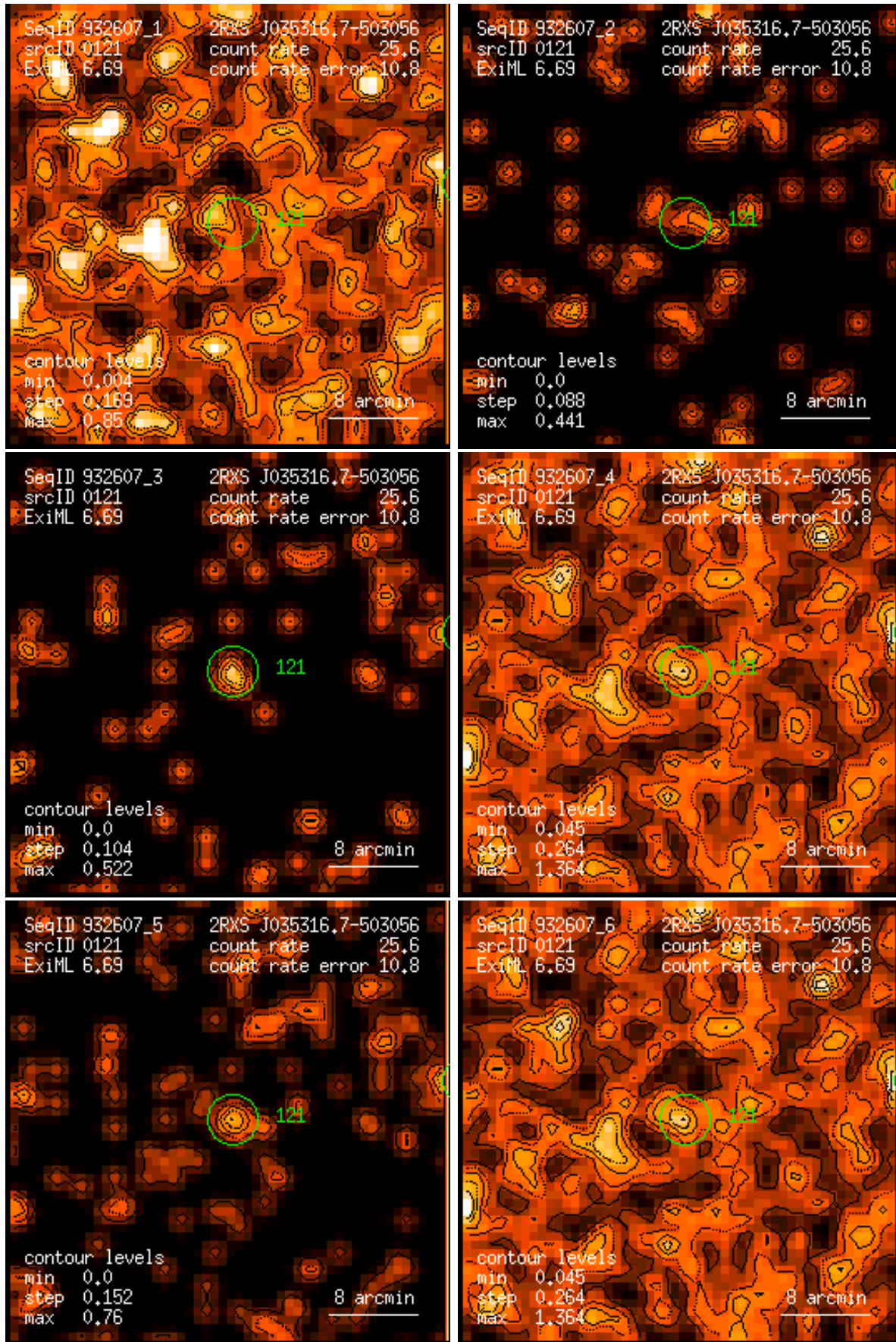
Figure 121: RASS 932607: detection 0121: band rate images, Gaussian filter: (1) PSPC channels 11 – 41, (2) 52 – 90, (3) 91 – 201, (4) 11 – 235, (5) 52 – 201, (6) 11 – 201. Broad band rates in counts/ks. Band rate contour levels in counts/ks/arcmin 2 .
