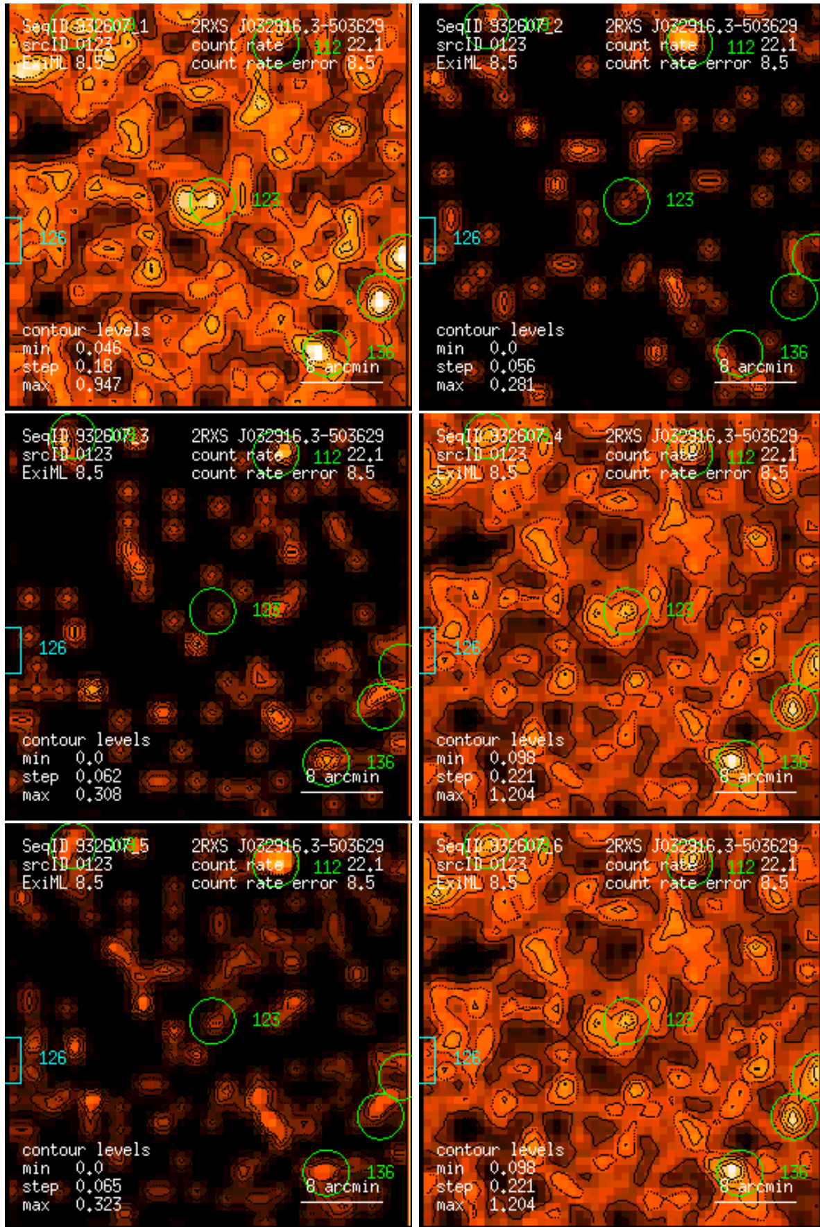
Figure 123: RASS 932607: detection 0123: band rate images, Gaussian filter: (1) PSPC channels 11 – 41, (2) 52 – 90, (3) 91 – 201, (4) 11 – 235, (5) 52 – 201, (6) 11 – 201. Broad band rates in counts/ks. Band rate contour levels in counts/ks/arcmin 2 .
