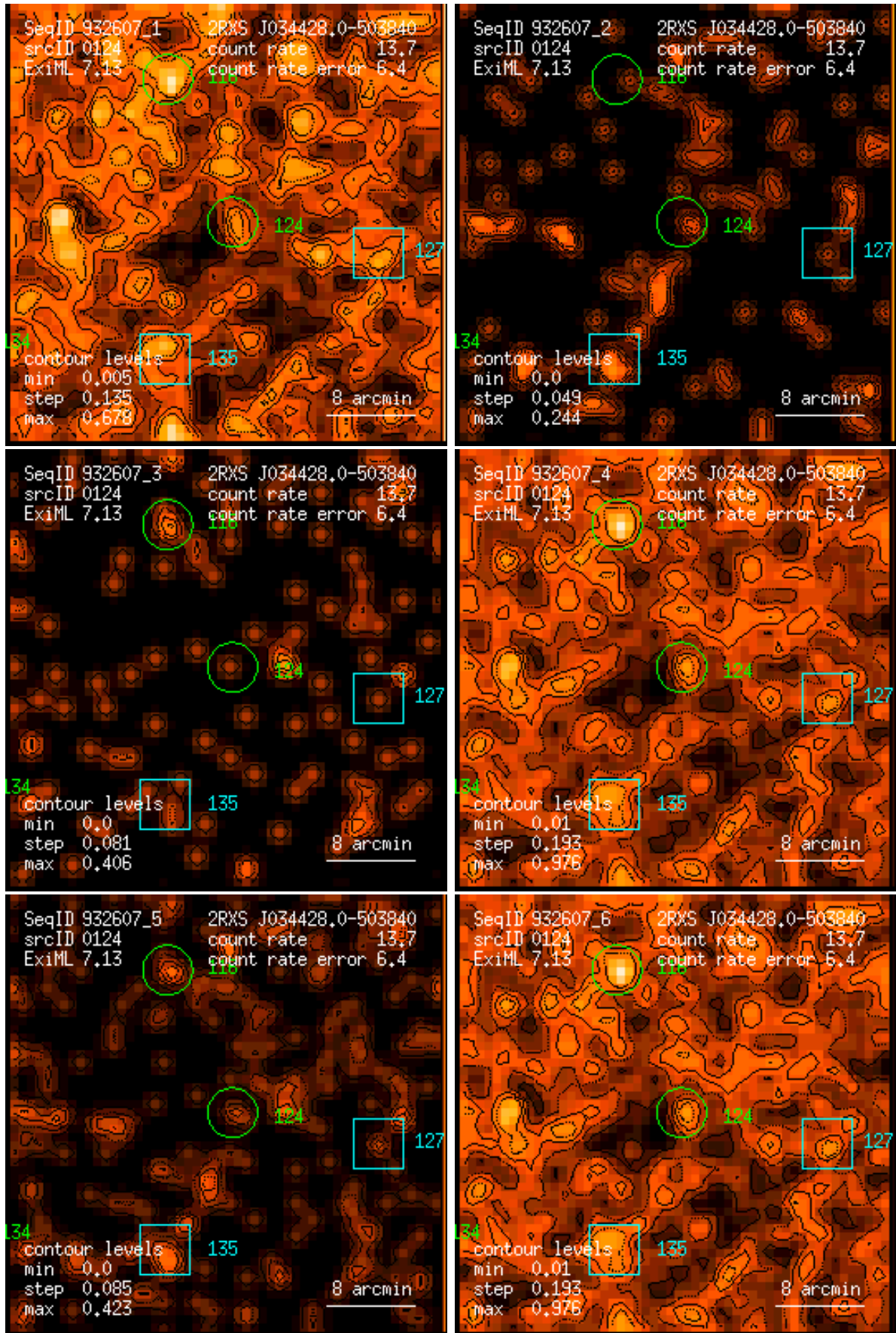
Figure 124: RASS 932607: detection 0124: band rate images, Gaussian filter: (1) PSPC channels 11 – 41, (2) 52 – 90, (3) 91 – 201, (4) 11 – 235, (5) 52 – 201, (6) 11 – 201. Broad band rates in counts/ks. Band rate contour levels in counts/ks/arcmin 2 .
