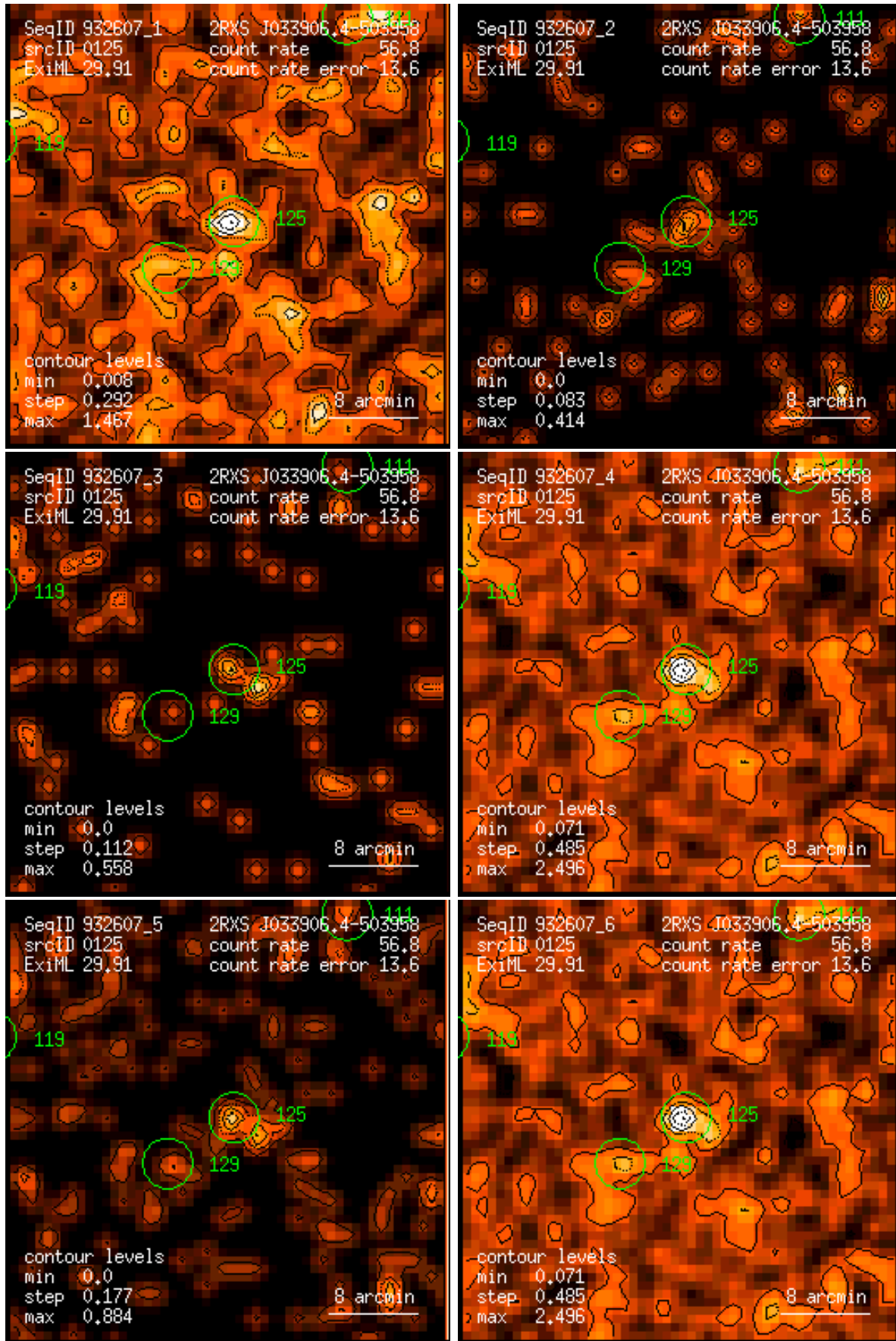
Figure 125: RASS 932607: detection 0125: band rate images, Gaussian filter: (1) PSPC channels 11 – 41, (2) 52 – 90, (3) 91 – 201, (4) 11 – 235, (5) 52 – 201, (6) 11 – 201. Broad band rates in counts/ks. Band rate contour levels in counts/ks/arcmin 2 .
