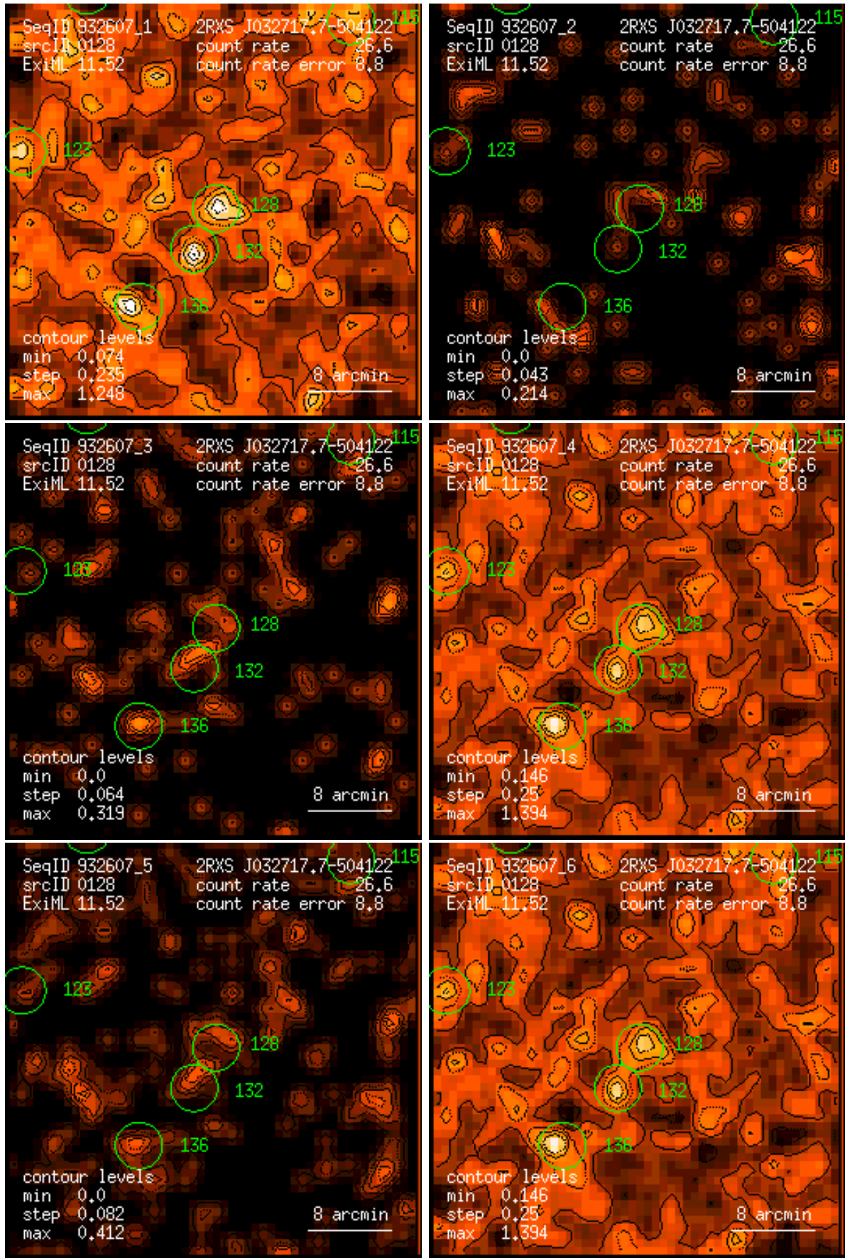
Figure 128: RASS 932607: detection 0128: band rate images, Gaussian filter: (1) PSPC channels 11 – 41, (2) 52 – 90, (3) 91 – 201, (4) 11 – 235, (5) 52 – 201, (6) 11 – 201. Broad band rates in counts/ks. Band rate contour levels in counts/ks/arcmin 2 .
