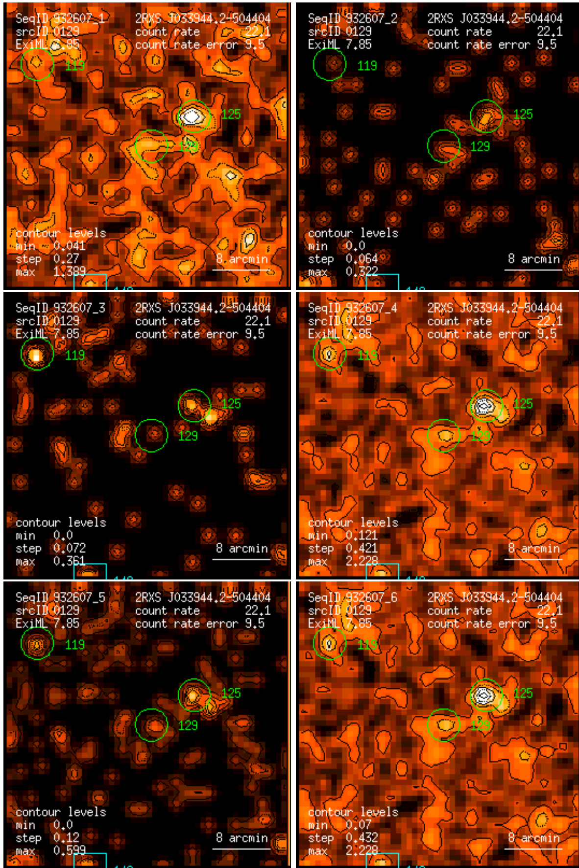
Figure 129: RASS 932607: detection 0129: band rate images, Gaussian filter: (1) PSPC channels 11 – 41, (2) 52 – 90, (3) 91 – 201, (4) 11 – 235, (5) 52 – 201, (6) 11 – 201. Broad band rates in counts/ks. Band rate contour levels in counts/ks/arcmin 2 .
