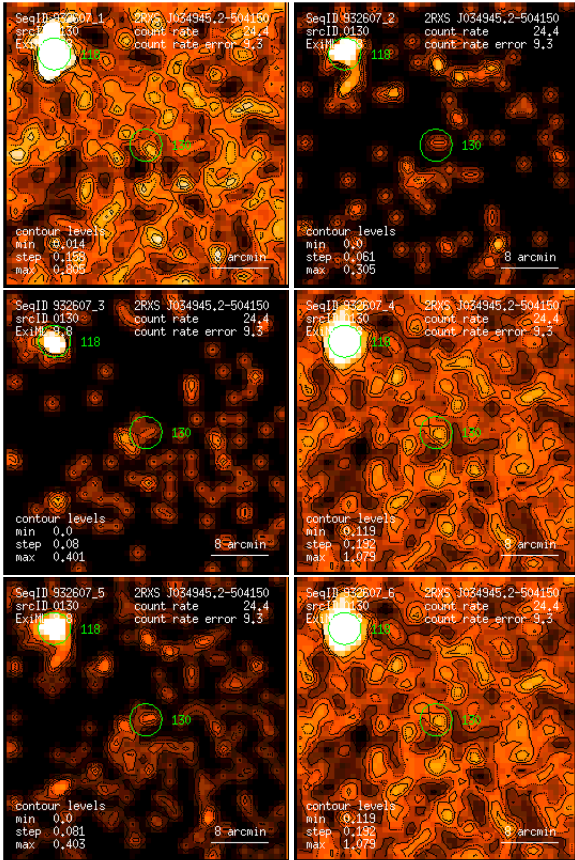
Figure 130: RASS 932607: detection 0130: band rate images, Gaussian filter: (1) PSPC channels 11 – 41, (2) 52 – 90, (3) 91 – 201, (4) 11 – 235, (5) 52 – 201, (6) 11 – 201. Broad band rates in counts/ks. Band rate contour levels in counts/ks/arcmin 2 .
