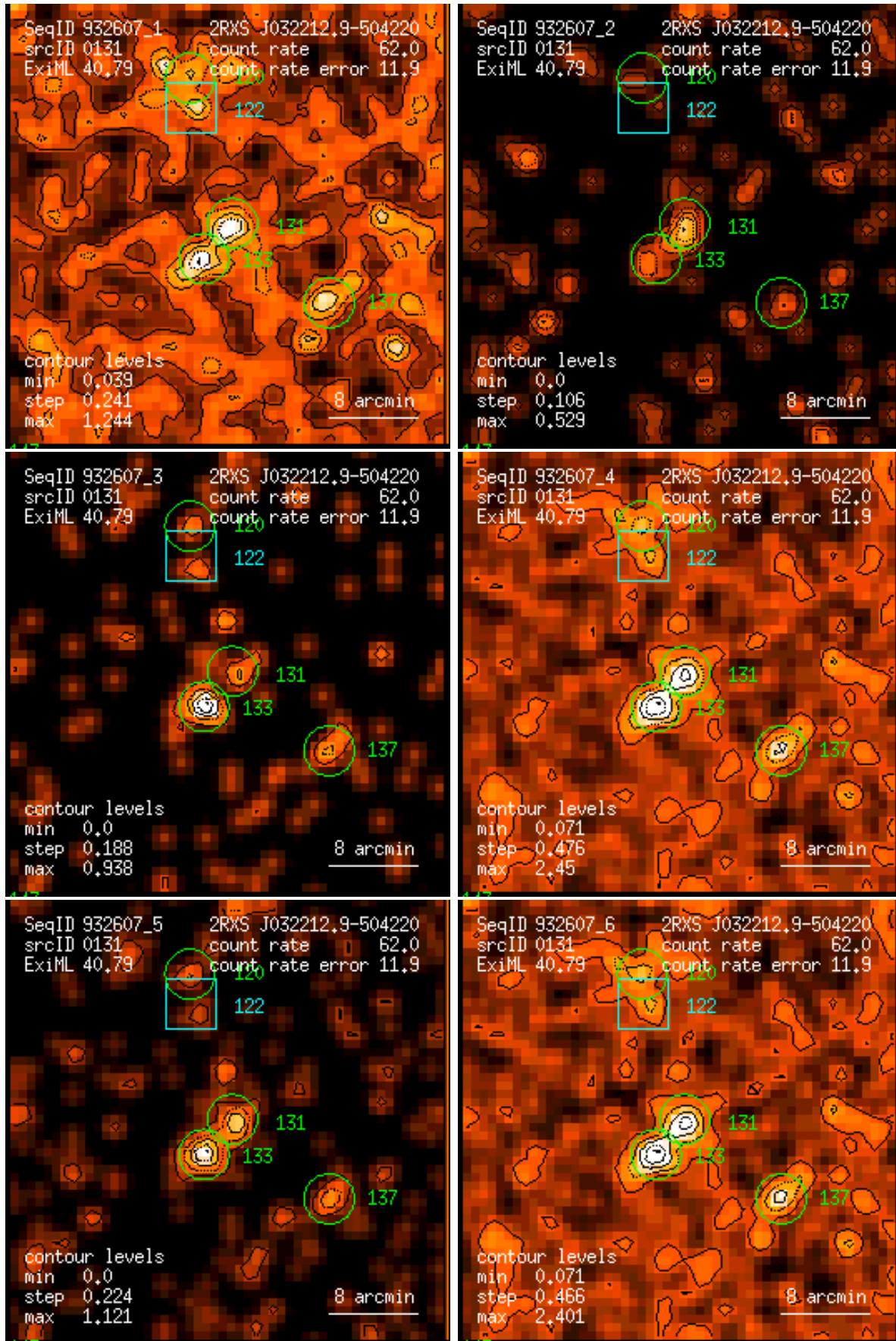
Figure 131: RASS 932607: detection 0131: band rate images, Gaussian filter: (1) PSPC channels 11 – 41, (2) 52 – 90, (3) 91 – 201, (4) 11 – 235, (5) 52 – 201, (6) 11 – 201. Broad band rates in counts/ks. Band rate contour levels in counts/ks/arcmin 2 .
