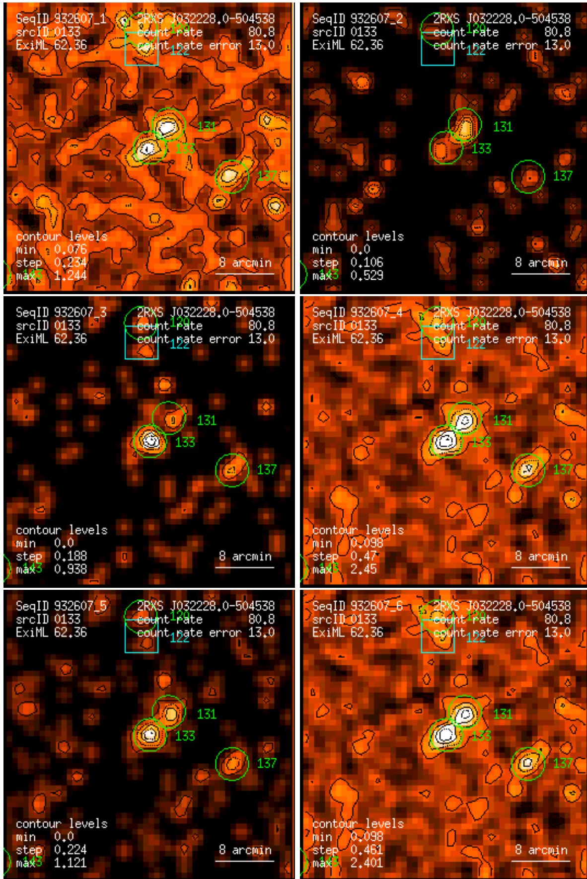
Figure 133: RASS 932607: detection 0133: band rate images, Gaussian filter: (1) PSPC channels 11 – 41, (2) 52 – 90, (3) 91 – 201, (4) 11 – 235, (5) 52 – 201, (6) 11 – 201. Broad band rates in counts/ks. Band rate contour levels in counts/ks/arcmin 2 .
