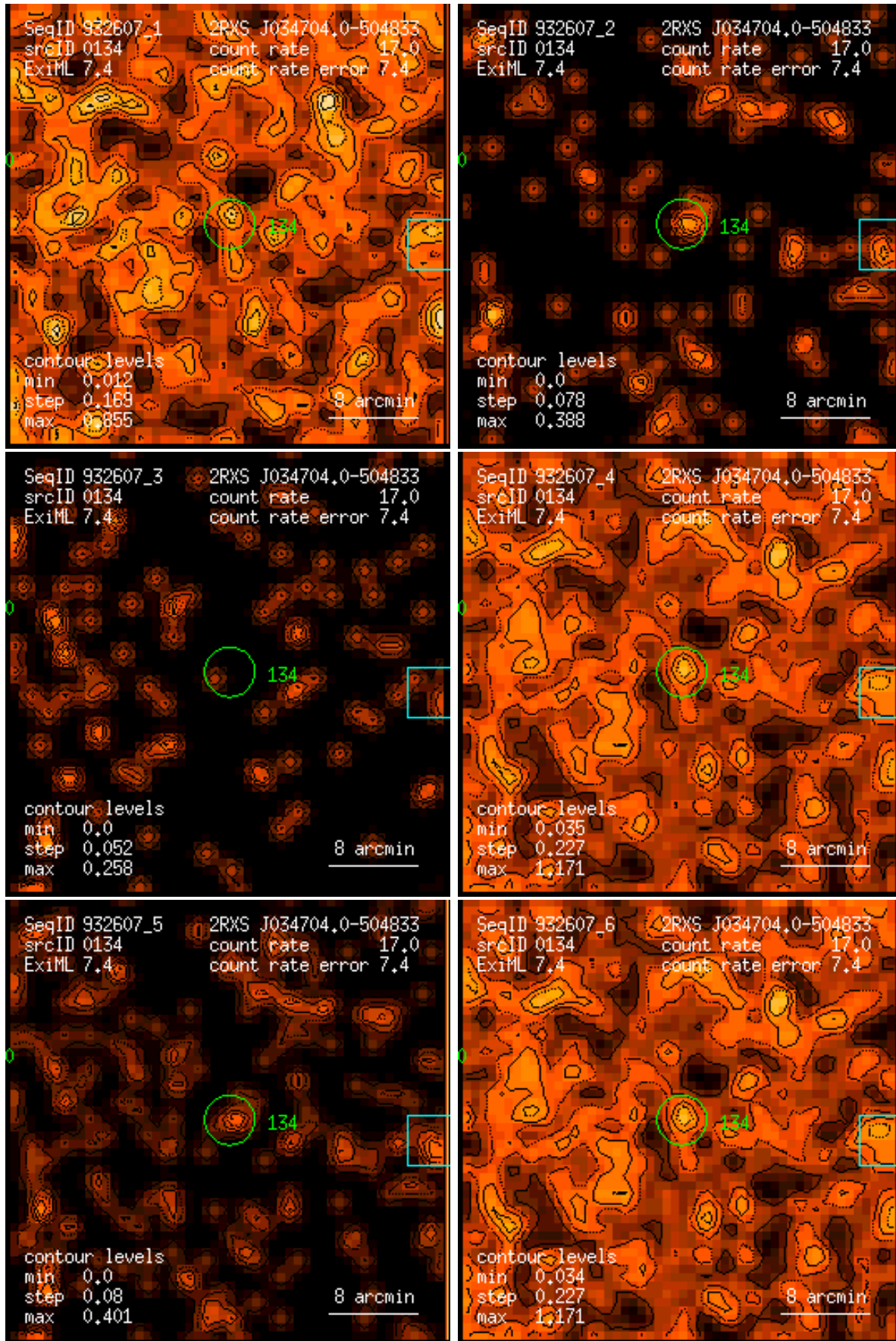
Figure 134: RASS 932607: detection 0134: band rate images, Gaussian filter: (1) PSPC channels 11 – 41, (2) 52 – 90, (3) 91 – 201, (4) 11 – 235, (5) 52 – 201, (6) 11 – 201. Broad band rates in counts/ks. Band rate contour levels in counts/ks/arcmin 2 .
