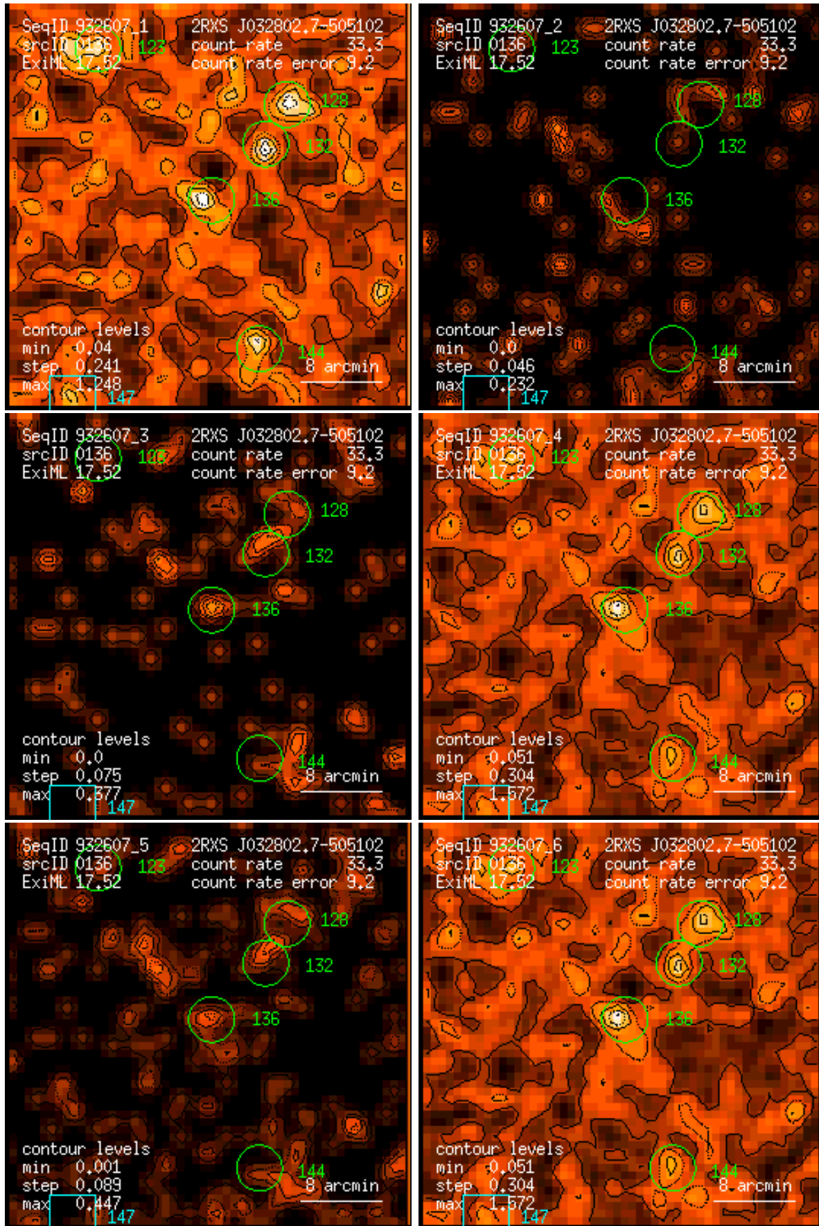
Figure 136: RASS 932607: detection 0136: band rate images, Gaussian filter: (1) PSPC channels 11 – 41, (2) 52 – 90, (3) 91 – 201, (4) 11 – 235, (5) 52 – 201, (6) 11 – 201. Broad band rates in counts/ks. Band rate contour levels in counts/ks/arcmin 2 .
