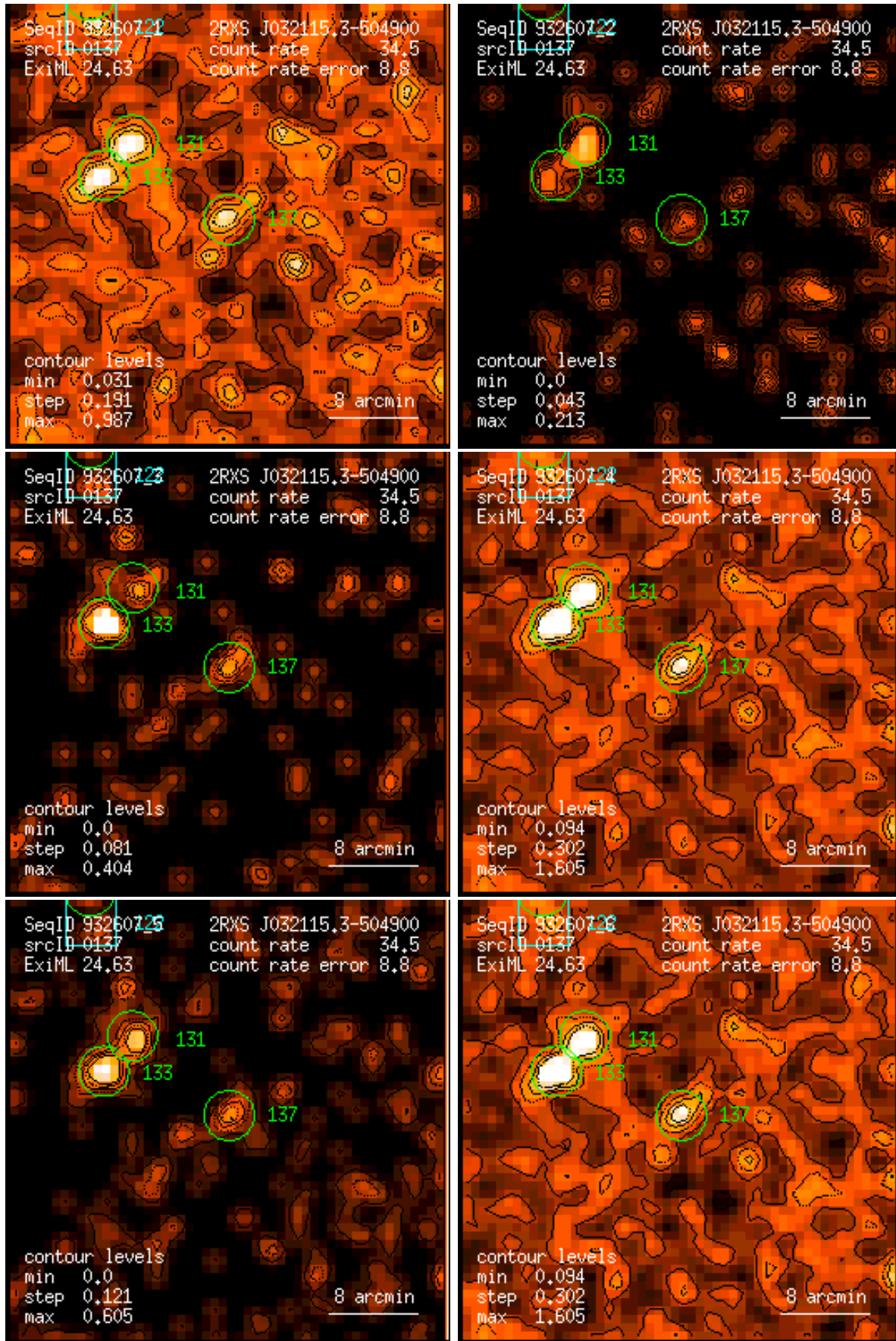
Figure 137: RASS 932607: detection 0137: band rate images, Gaussian filter: (1) PSPC channels 11 – 41, (2) 52 – 90, (3) 91 – 201, (4) 11 – 235, (5) 52 – 201, (6) 11 – 201. Broad band rates in counts/ks. Band rate contour levels in counts/ks/arcmin 2 .
