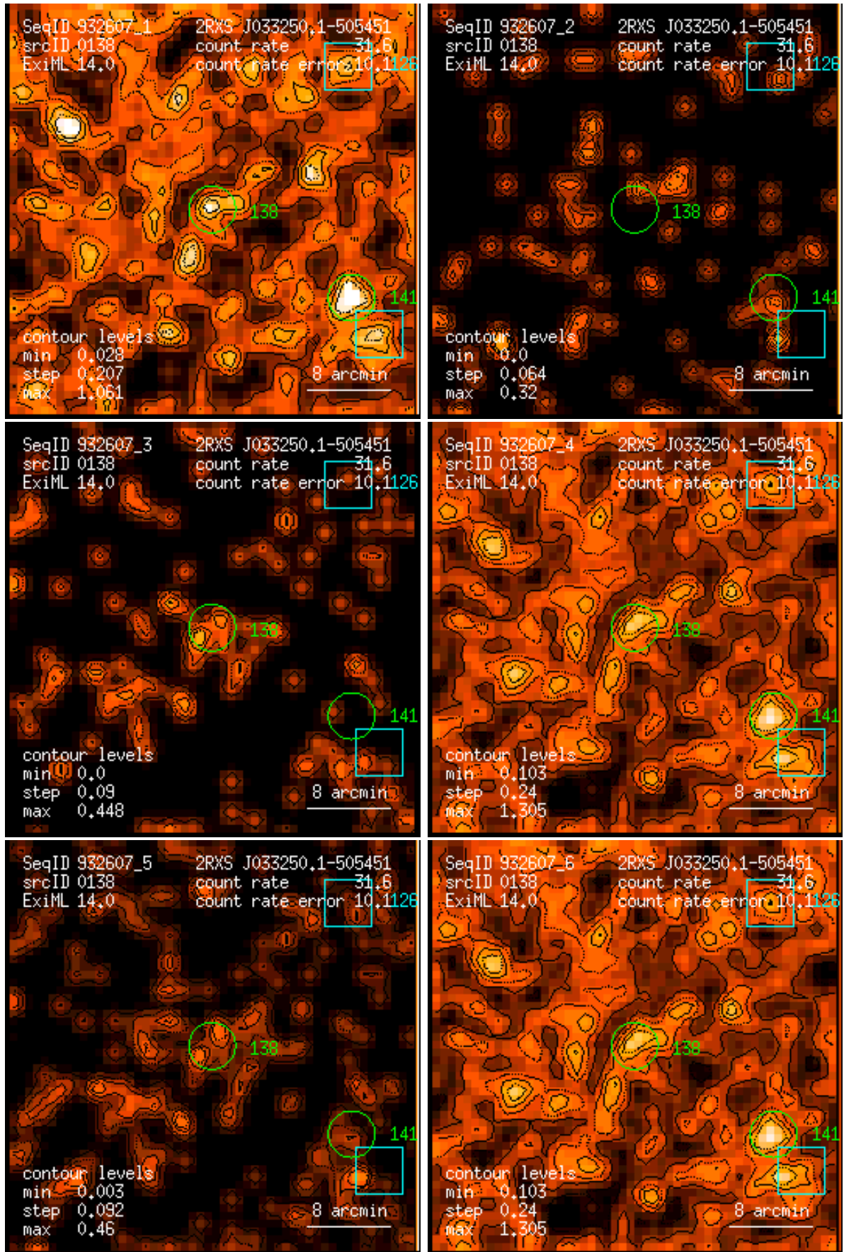
Figure 138: RASS 932607: detection 0138: band rate images, Gaussian filter: (1) PSPC channels 11 – 41, (2) 52 – 90, (3) 91 – 201, (4) 11 – 235, (5) 52 – 201, (6) 11 – 201. Broad band rates in counts/ks. Band rate contour levels in counts/ks/arcmin 2 .
