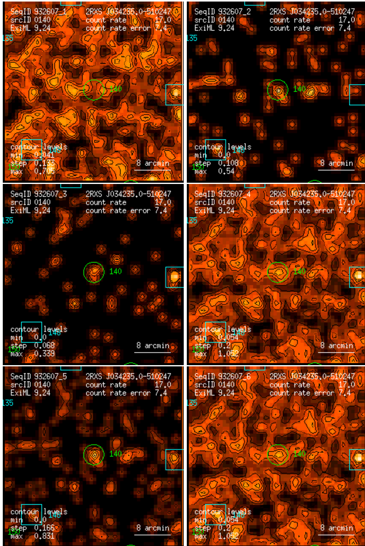
Figure 140: RASS 932607: detection 0140: band rate images, Gaussian filter: (1) PSPC channels 11 – 41, (2) 52 – 90, (3) 91 – 201, (4) 11 – 235, (5) 52 – 201, (6) 11 – 201. Broad band rates in counts/ks. Band rate contour levels in counts/ks/arcmin 2 .
