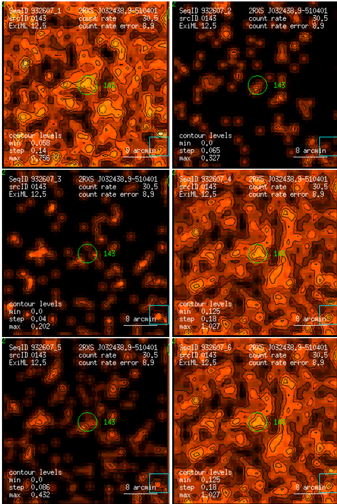
Figure 143: RASS 932607: detection 0143: band rate images, Gaussian filter: (1) PSPC channels 11 – 41, (2) 52 – 90, (3) 91 – 201, (4) 11 – 235, (5) 52 – 201, (6) 11 – 201. Broad band rates in counts/ks. Band rate contour levels in counts/ks/arcmin 2 .
