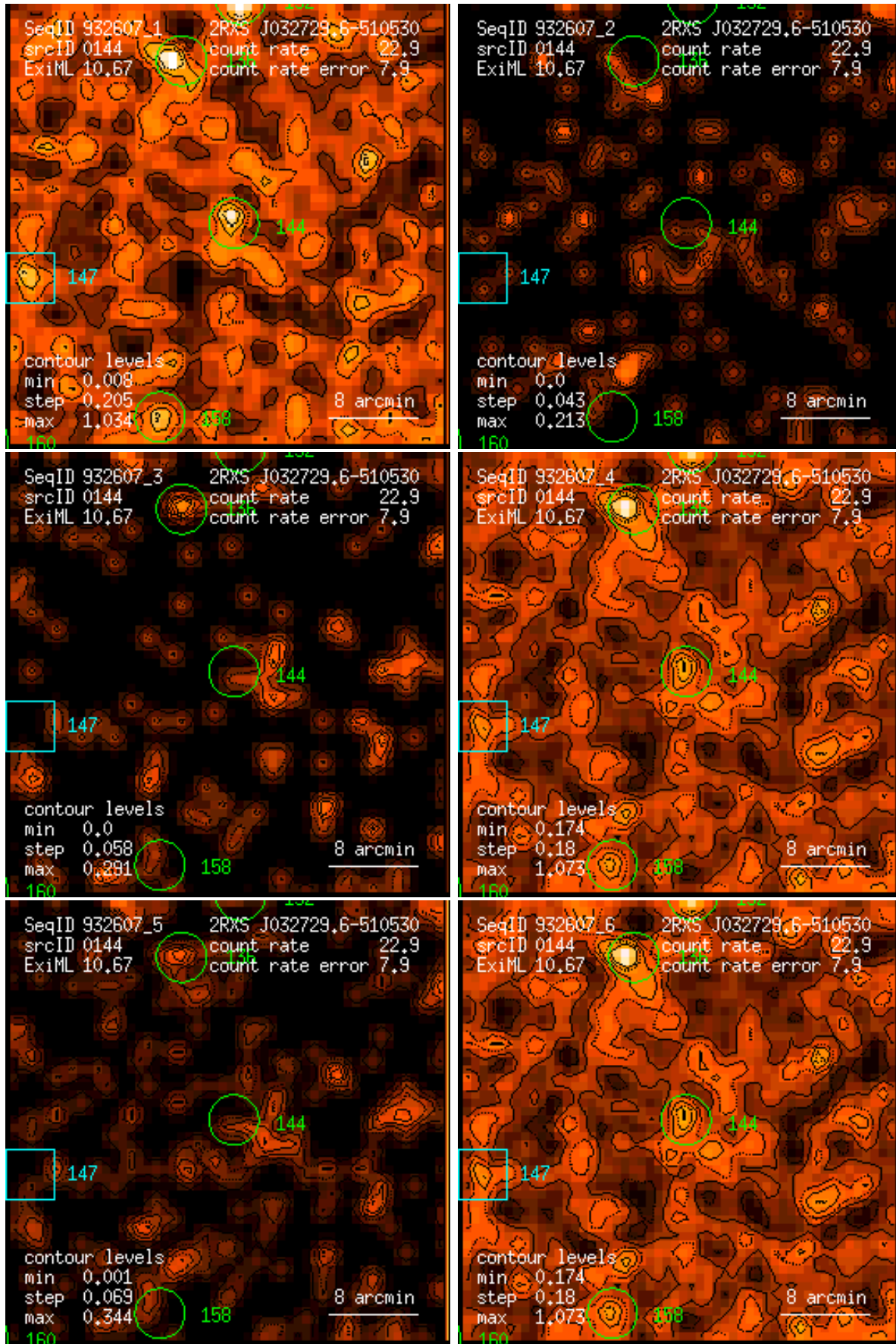
Figure 144: RASS 932607: detection 0144: band rate images, Gaussian filter: (1) PSPC channels 11 – 41, (2) 52 – 90, (3) 91 – 201, (4) 11 – 235, (5) 52 – 201, (6) 11 – 201. Broad band rates in counts/ks. Band rate contour levels in counts/ks/arcmin 2 .
