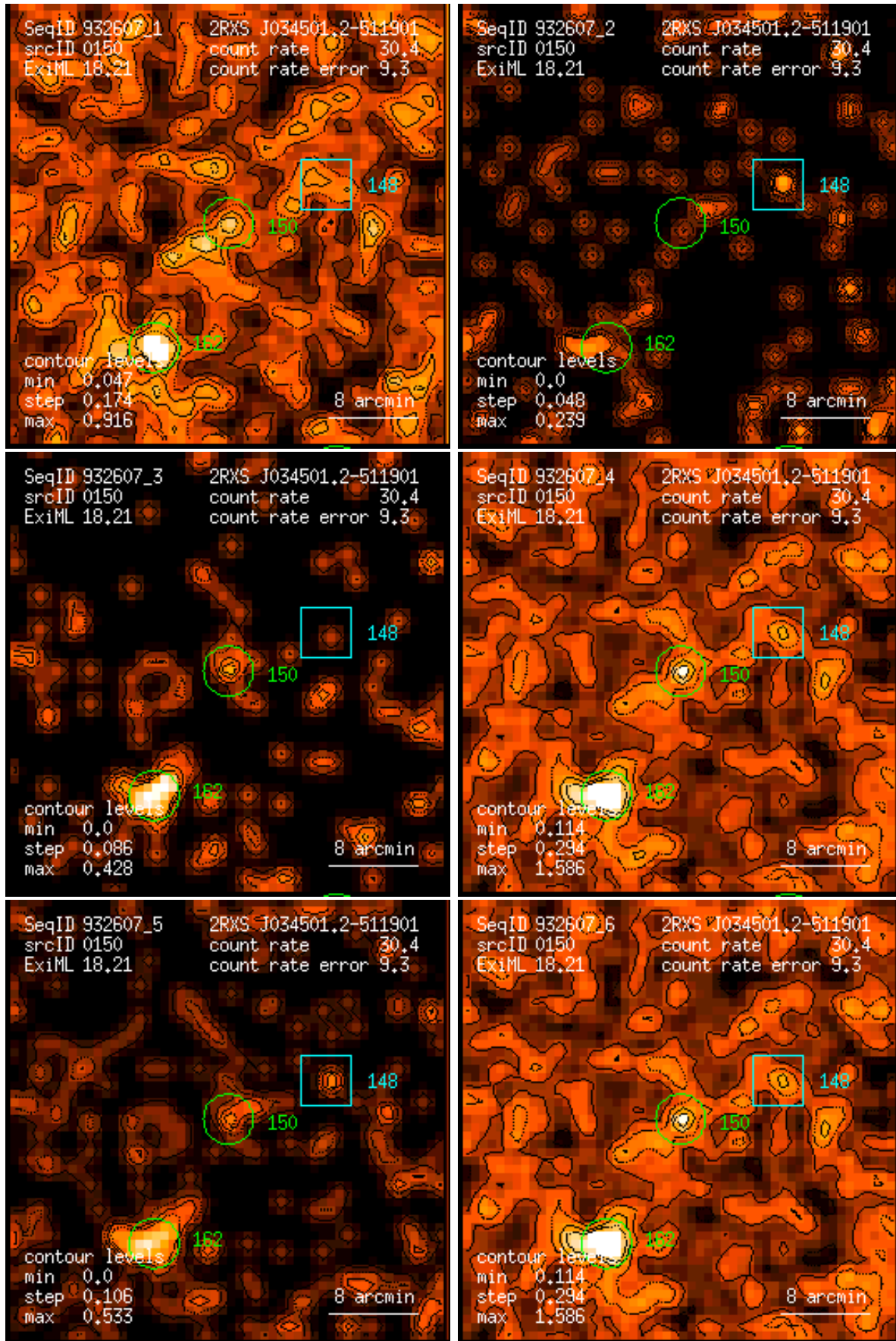
Figure 150: RASS 932607: detection 0150: band rate images, Gaussian filter: (1) PSPC channels 11 – 41, (2) 52 – 90, (3) 91 – 201, (4) 11 – 235, (5) 52 – 201, (6) 11 – 201. Broad band rates in counts/ks. Band rate contour levels in counts/ks/arcmin 2 .
