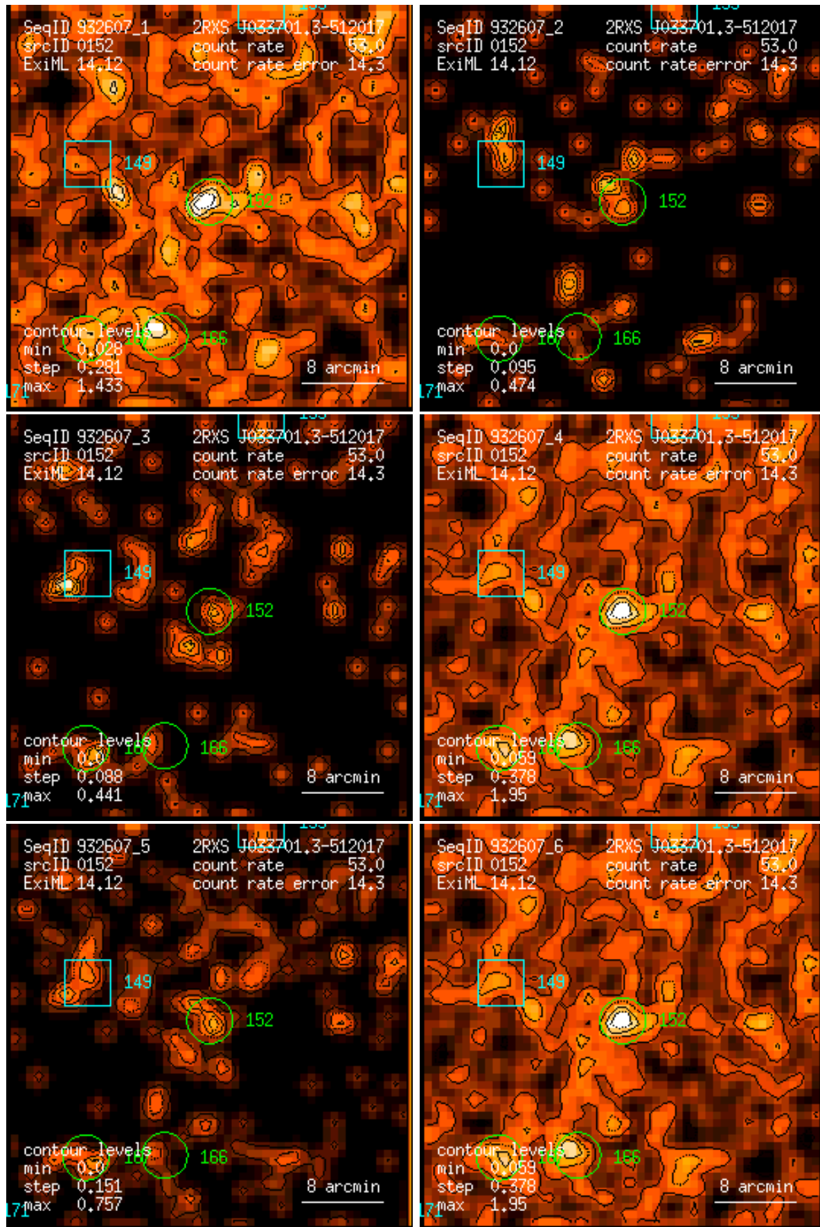
Figure 152: RASS 932607: detection 0152: band rate images, Gaussian filter: (1) PSPC channels 11 – 41, (2) 52 – 90, (3) 91 – 201, (4) 11 – 235, (5) 52 – 201, (6) 11 – 201. Broad band rates in counts/ks. Band rate contour levels in counts/ks/arcmin 2 .
