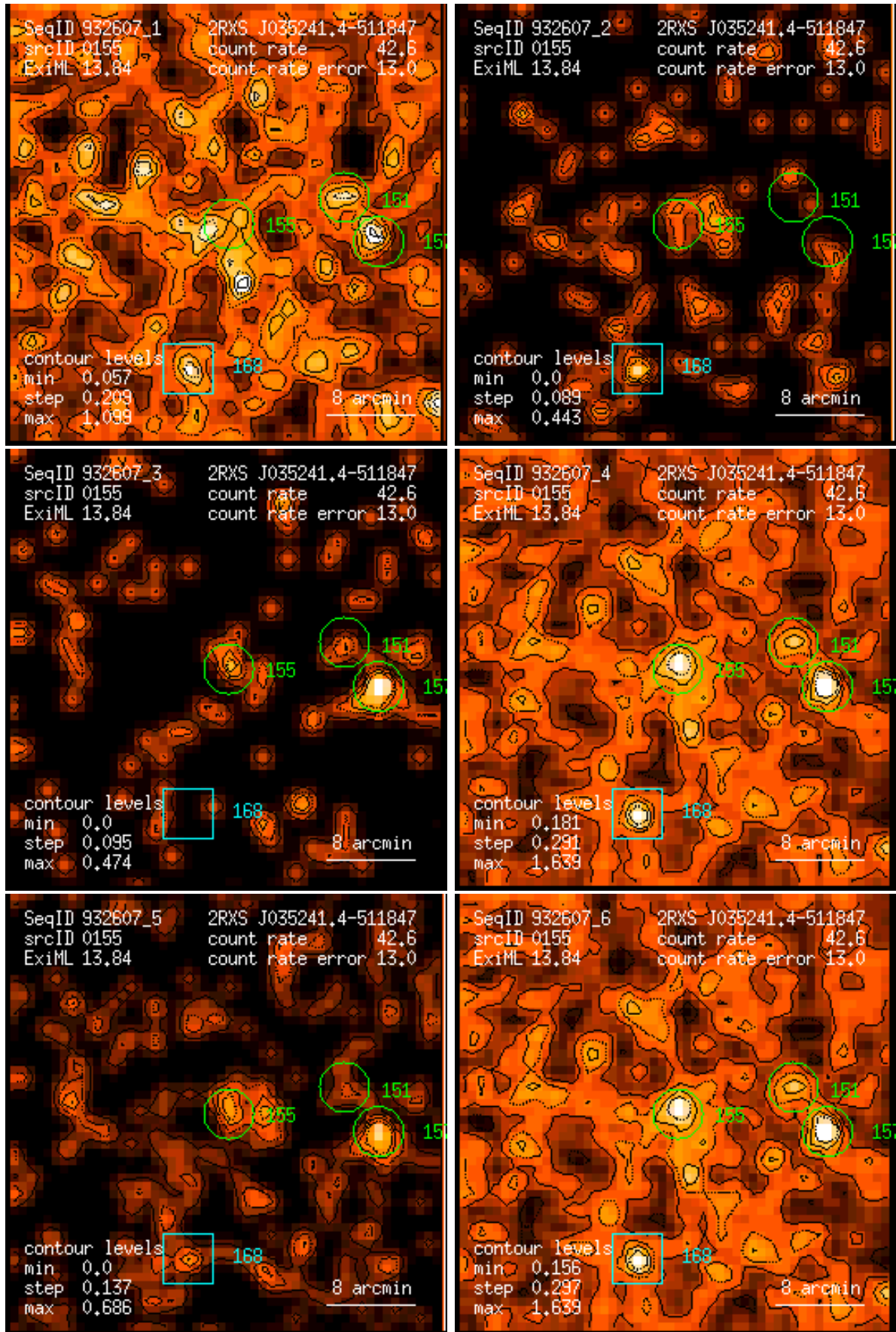
Figure 155: RASS 932607: detection 0155: band rate images, Gaussian filter: (1) PSPC channels 11 – 41, (2) 52 – 90, (3) 91 – 201, (4) 11 – 235, (5) 52 – 201, (6) 11 – 201. Broad band rates in counts/ks. Band rate contour levels in counts/ks/arcmin 2 .
