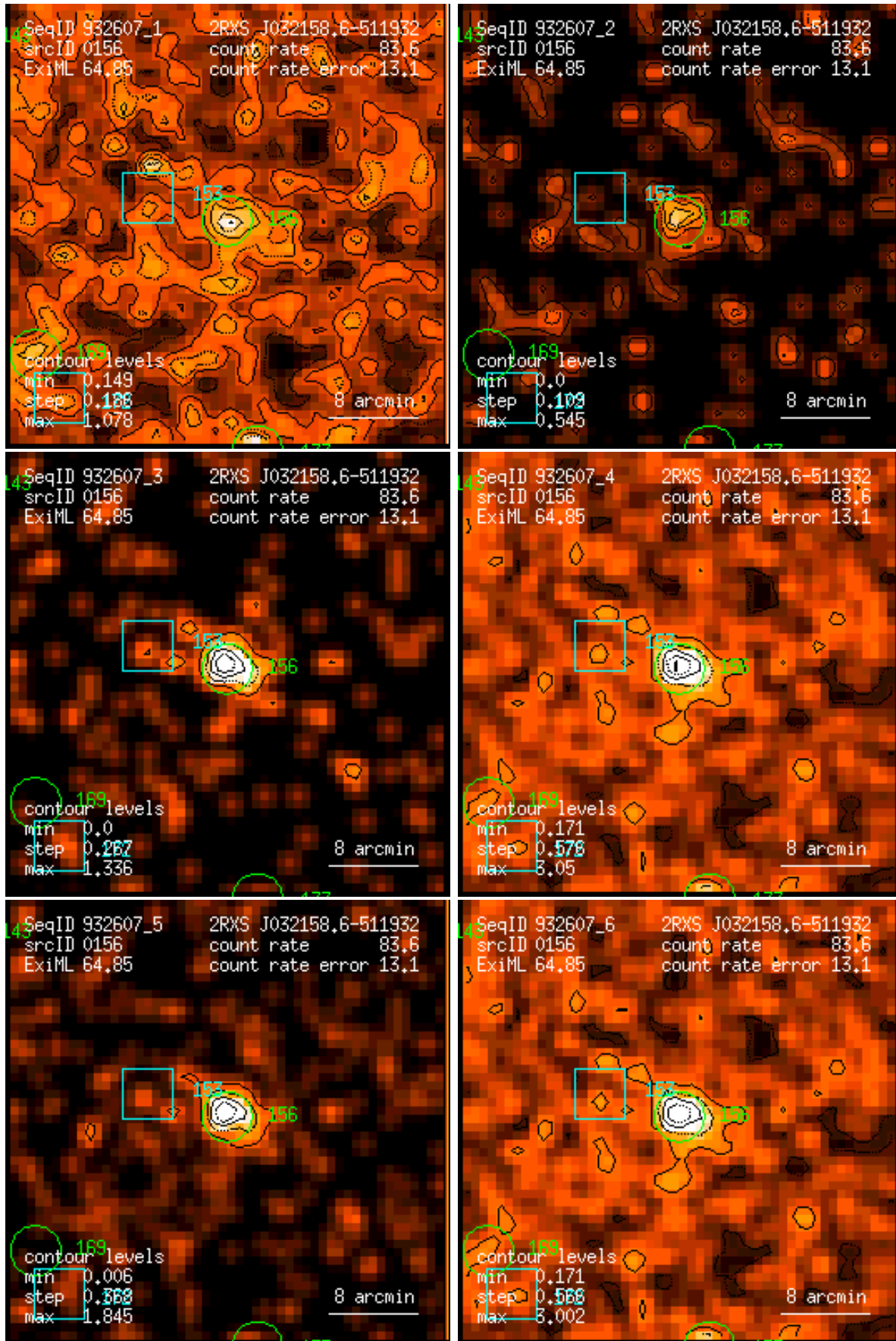
Figure 156: RASS 932607: detection 0156: band rate images, Gaussian filter: (1) PSPC channels 11 – 41, (2) 52 – 90, (3) 91 – 201, (4) 11 – 235, (5) 52 – 201, (6) 11 – 201. Broad band rates in counts/ks. Band rate contour levels in counts/ks/arcmin 2 .
