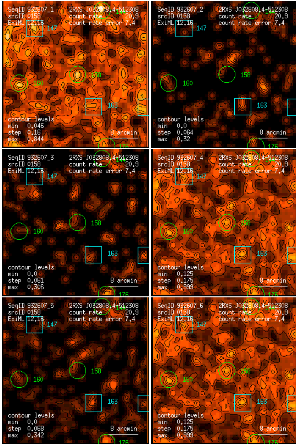
Figure 158: RASS 932607: detection 0158: band rate images, Gaussian filter: (1) PSPC channels 11 – 41, (2) 52 – 90, (3) 91 – 201, (4) 11 – 235, (5) 52 – 201, (6) 11 – 201. Broad band rates in counts/ks. Band rate contour levels in counts/ks/arcmin 2 .
