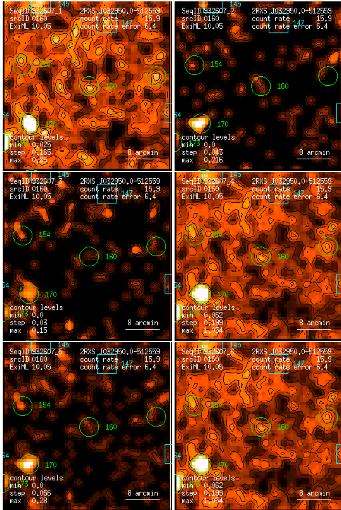
Figure 160: RASS 932607: detection 0160: band rate images, Gaussian filter: (1) PSPC channels 11 – 41, (2) 52 – 90, (3) 91 – 201, (4) 11 – 235, (5) 52 – 201, (6) 11 – 201. Broad band rates in counts/ks. Band rate contour levels in counts/ks/arcmin 2 .
