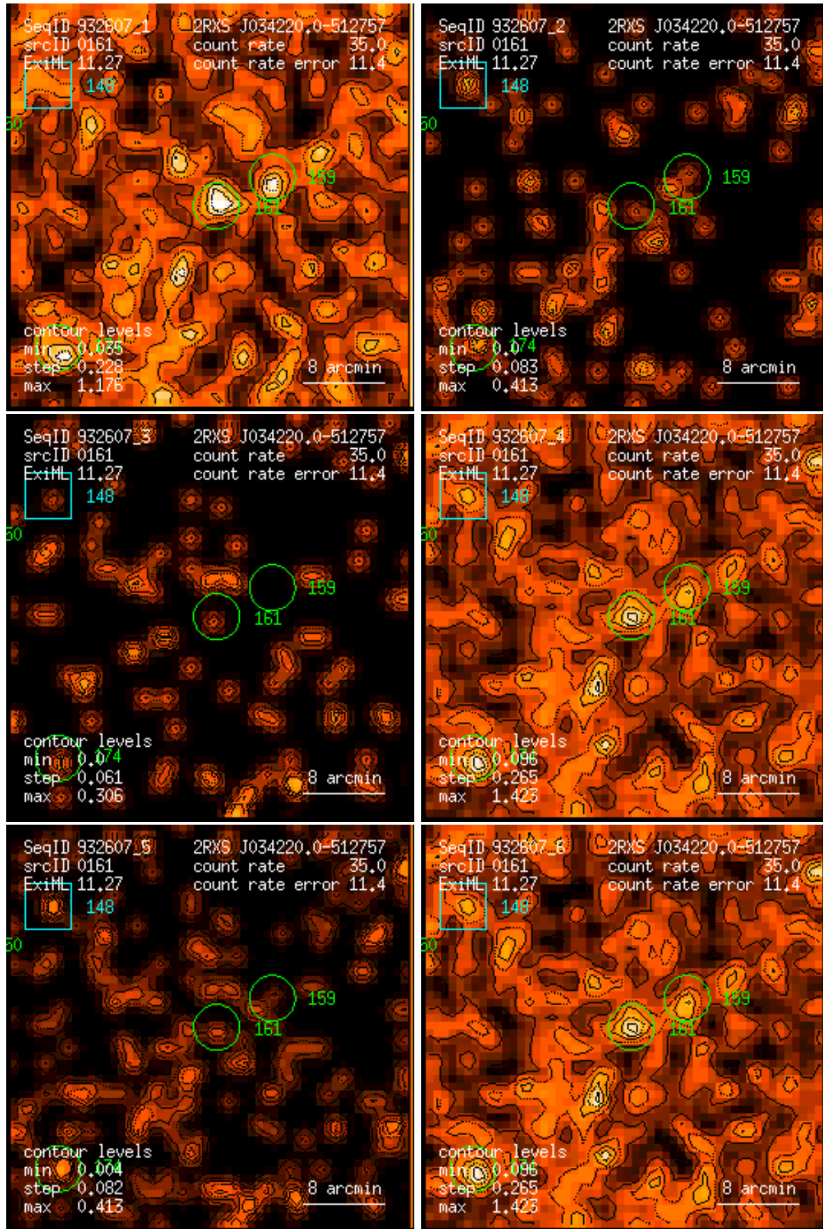
Figure 161: RASS 932607: detection 0161: band rate images, Gaussian filter: (1) PSPC channels 11 – 41, (2) 52 – 90, (3) 91 – 201, (4) 11 – 235, (5) 52 – 201, (6) 11 – 201. Broad band rates in counts/ks. Band rate contour levels in counts/ks/arcmin 2 .
