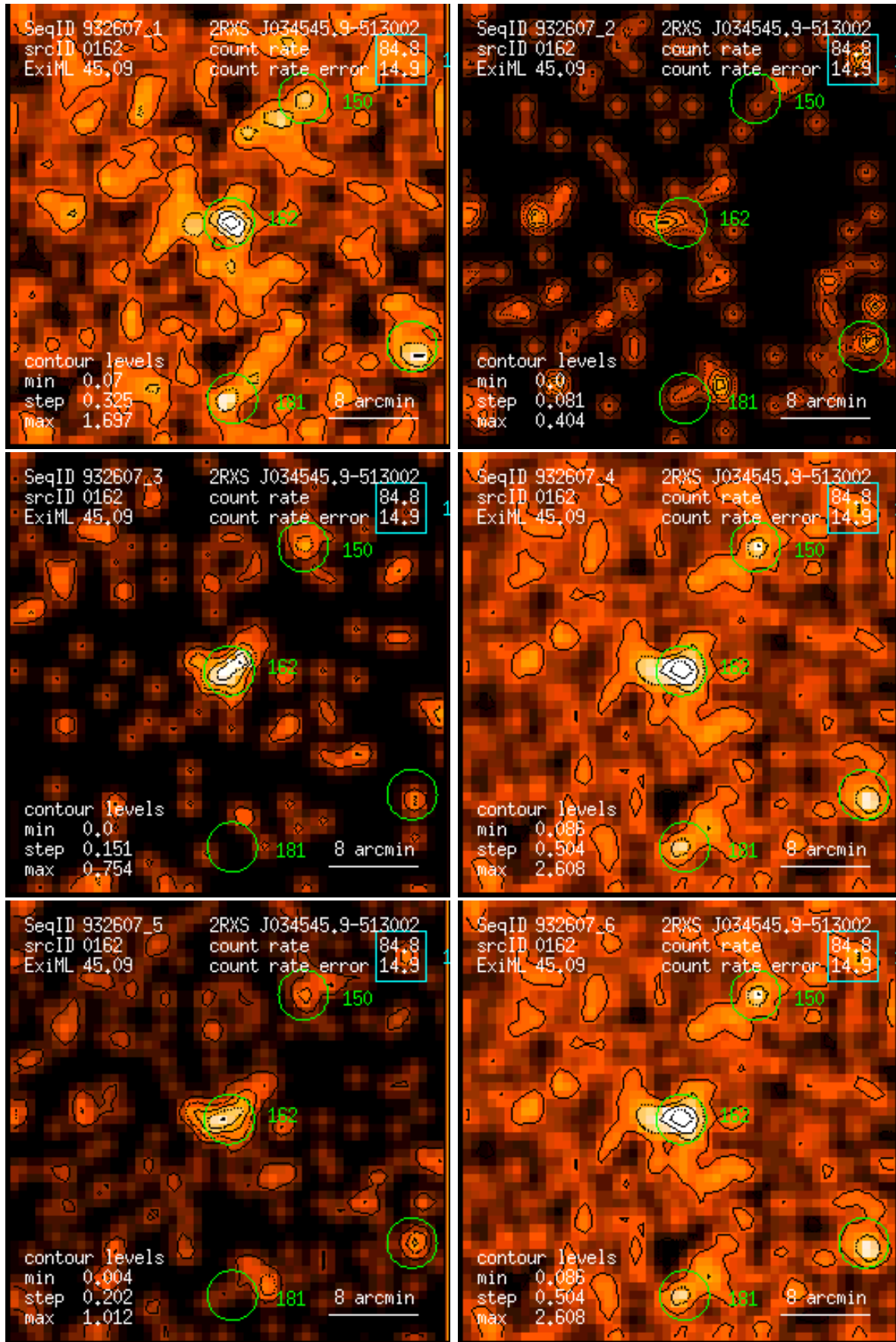
Figure 162: RASS 932607: detection 0162: band rate images, Gaussian filter: (1) PSPC channels 11 – 41, (2) 52 – 90, (3) 91 – 201, (4) 11 – 235, (5) 52 – 201, (6) 11 – 201. Broad band rates in counts/ks. Band rate contour levels in counts/ks/arcmin 2 .
