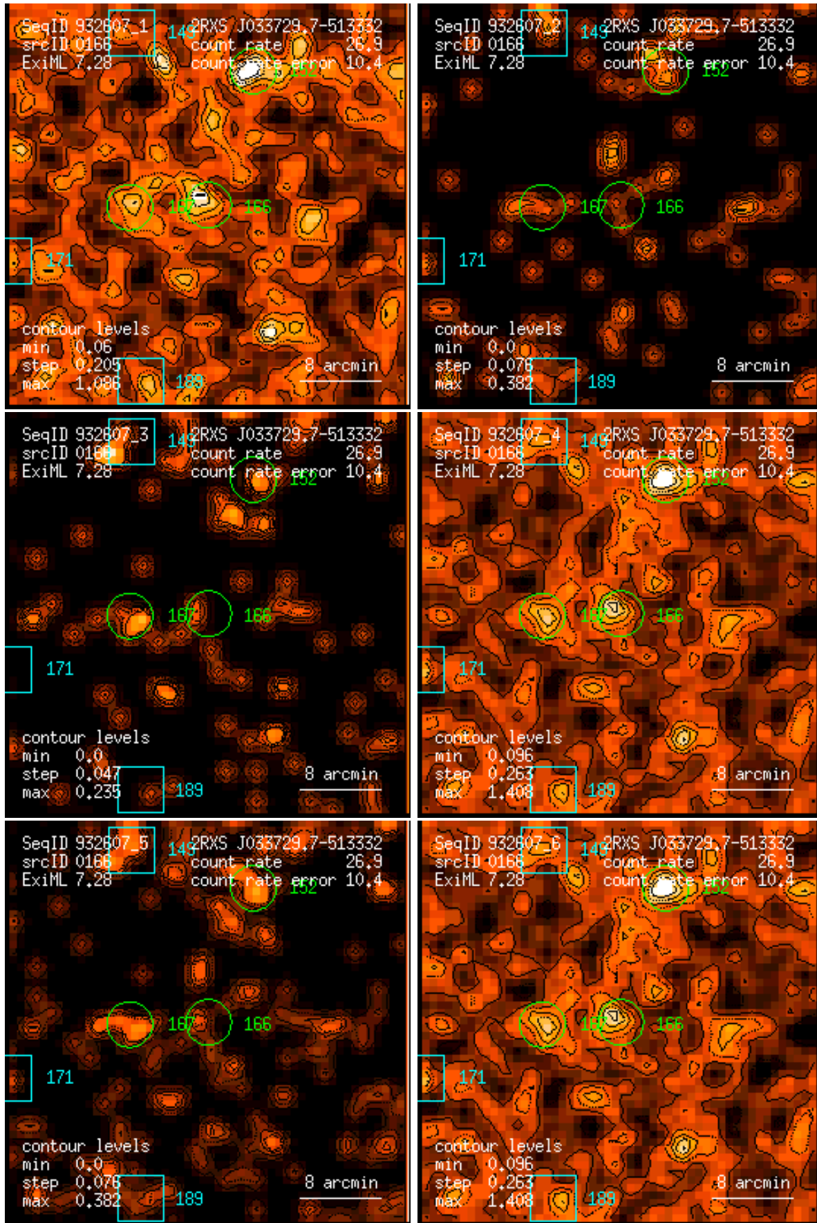
Figure 166: RASS 932607: detection 0166: band rate images, Gaussian filter: (1) PSPC channels 11 – 41, (2) 52 – 90, (3) 91 – 201, (4) 11 – 235, (5) 52 – 201, (6) 11 – 201. Broad band rates in counts/ks. Band rate contour levels in counts/ks/arcmin 2 .
