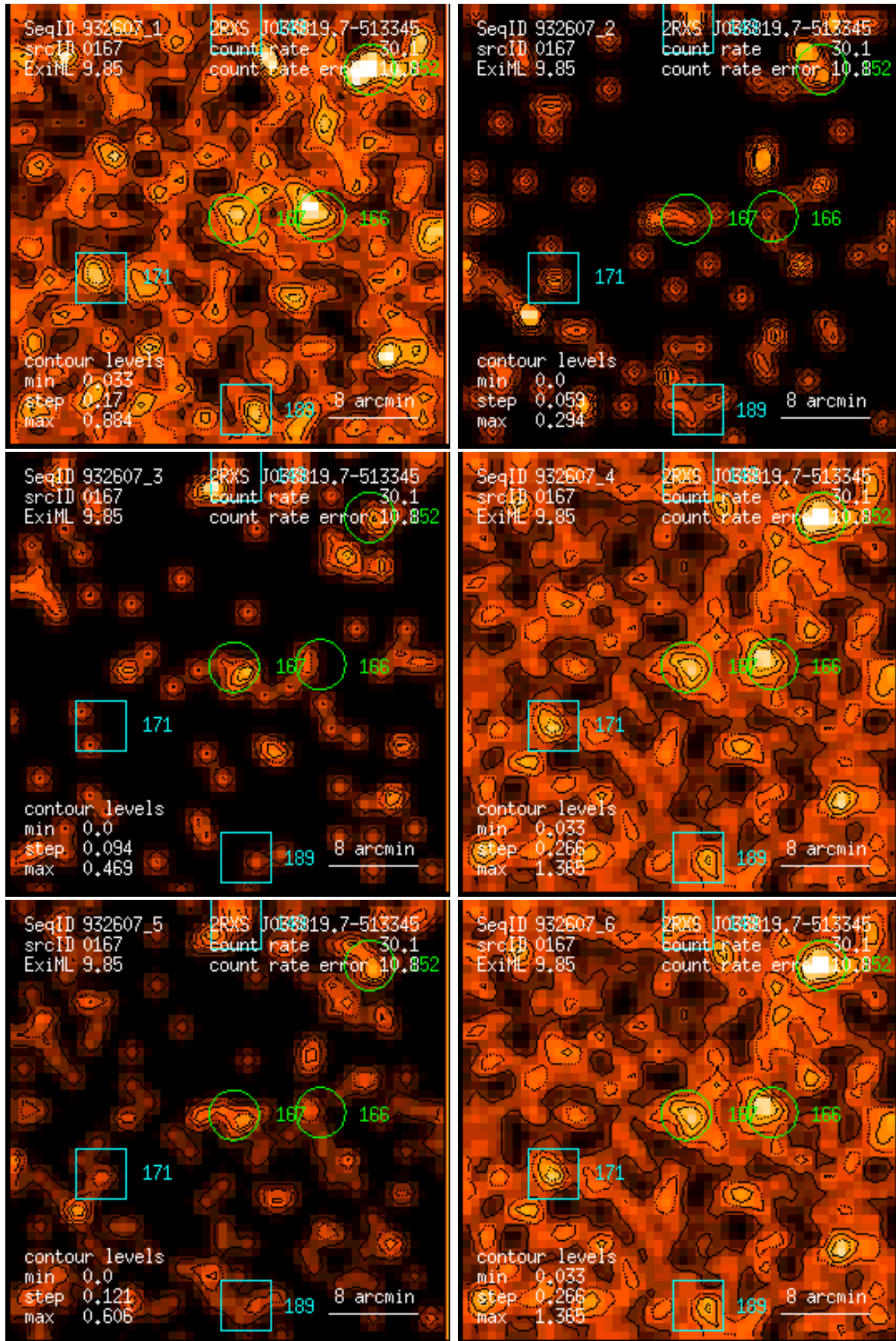
Figure 167: RASS 932607: detection 0167: band rate images, Gaussian filter: (1) PSPC channels 11 – 41, (2) 52 – 90, (3) 91 – 201, (4) 11 – 235, (5) 52 – 201, (6) 11 – 201. Broad band rates in counts/ks. Band rate contour levels in counts/ks/arcmin 2 .
