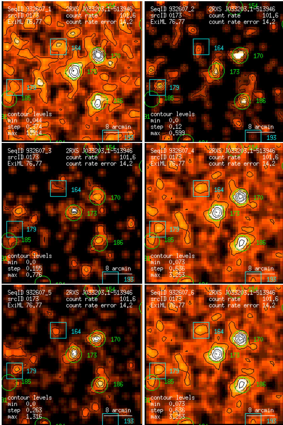
Figure 173: RASS 932607: detection 0173: band rate images, Gaussian filter: (1) PSPC channels 11 – 41, (2) 52 – 90, (3) 91 – 201, (4) 11 – 235, (5) 52 – 201, (6) 11 – 201. Broad band rates in counts/ks. Band rate contour levels in counts/ks/arcmin 2 .
