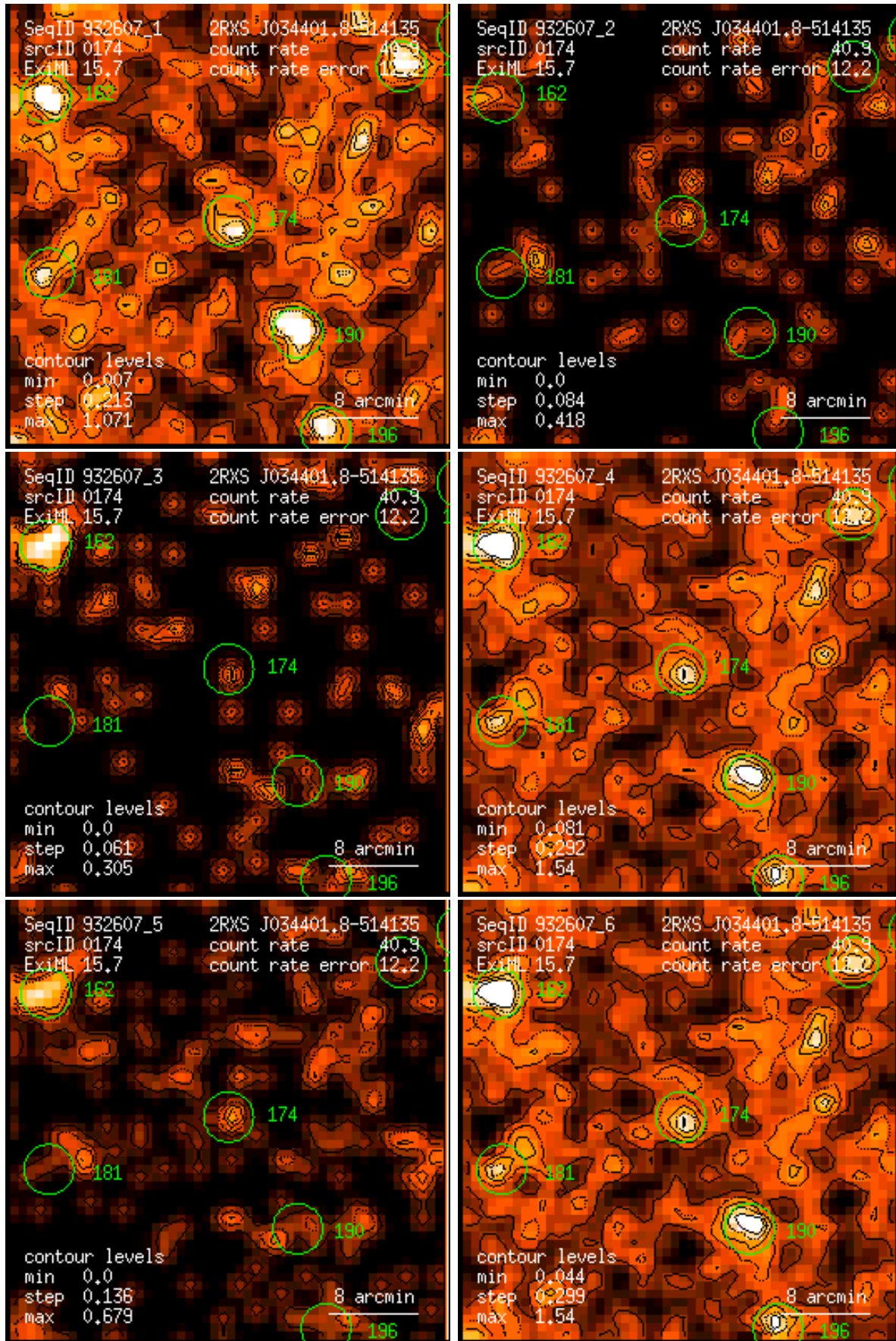
Figure 174: RASS 932607: detection 0174: band rate images, Gaussian filter: (1) PSPC channels 11 – 41, (2) 52 – 90, (3) 91 – 201, (4) 11 – 235, (5) 52 – 201, (6) 11 – 201. Broad band rates in counts/ks. Band rate contour levels in counts/ks/arcmin 2 .
