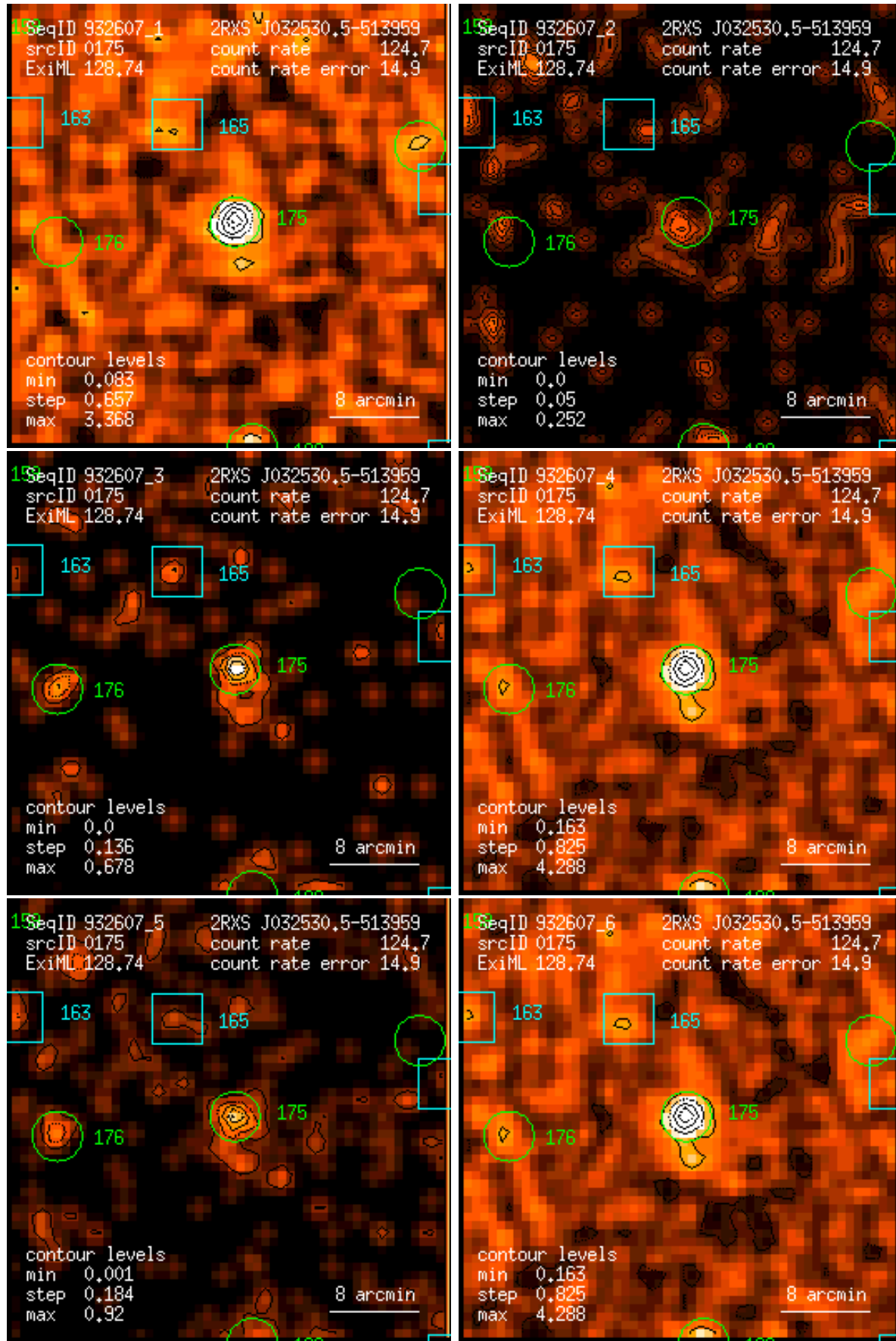
Figure 175: RASS 932607: detection 0175: band rate images, Gaussian filter: (1) PSPC channels 11 – 41, (2) 52 – 90, (3) 91 – 201, (4) 11 – 235, (5) 52 – 201, (6) 11 – 201. Broad band rates in counts/ks. Band rate contour levels in counts/ks/arcmin 2 .
