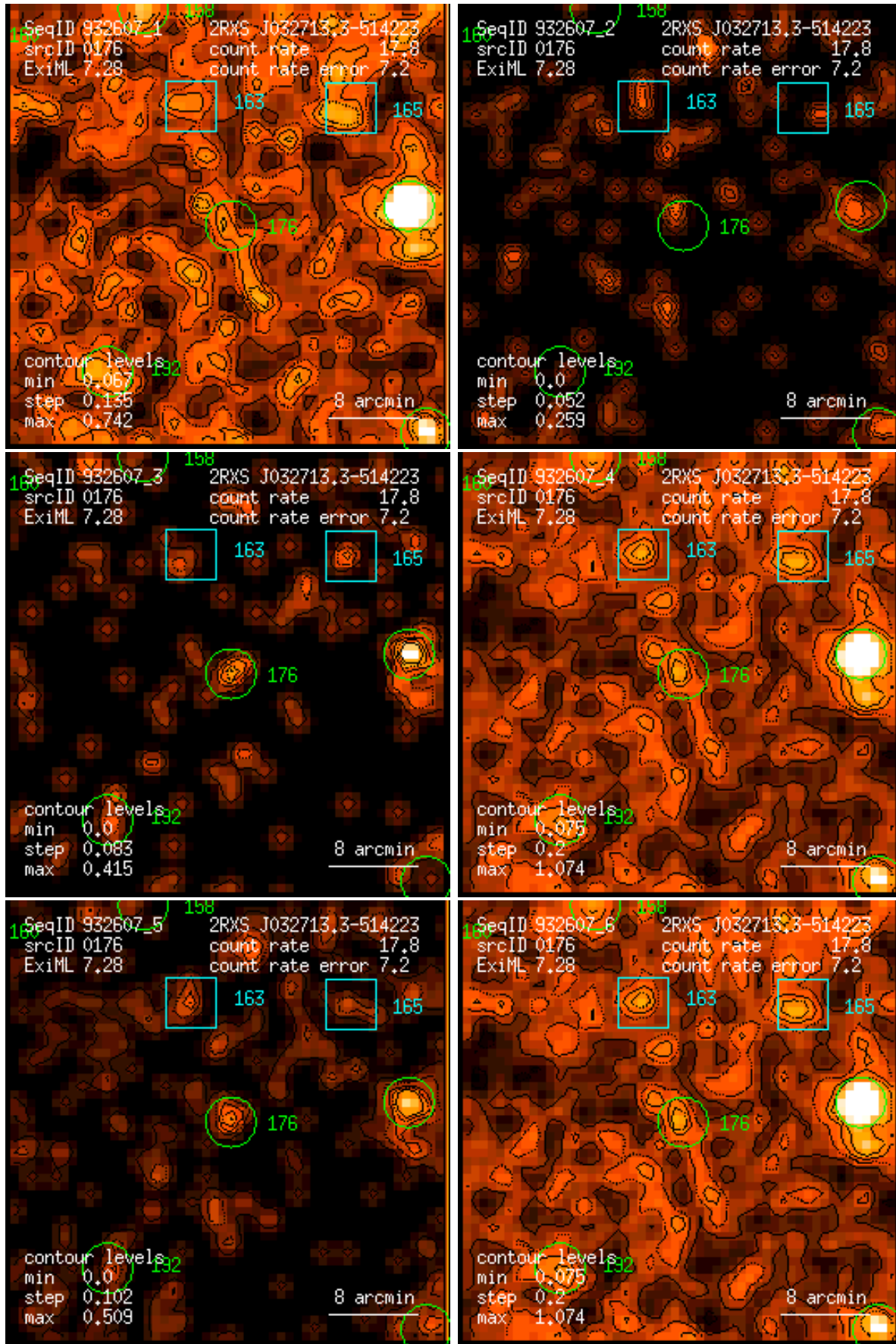
Figure 176: RASS 932607: detection 0176: band rate images, Gaussian filter: (1) PSPC channels 11 – 41, (2) 52 – 90, (3) 91 – 201, (4) 11 – 235, (5) 52 – 201, (6) 11 – 201. Broad band rates in counts/ks. Band rate contour levels in counts/ks/arcmin 2 .
