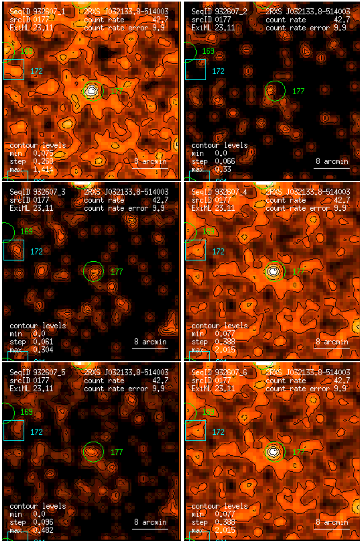
Figure 177: RASS 932607: detection 0177: band rate images, Gaussian filter: (1) PSPC channels 11 – 41, (2) 52 – 90, (3) 91 – 201, (4) 11 – 235, (5) 52 – 201, (6) 11 – 201. Broad band rates in counts/ks. Band rate contour levels in counts/ks/arcmin 2 .
