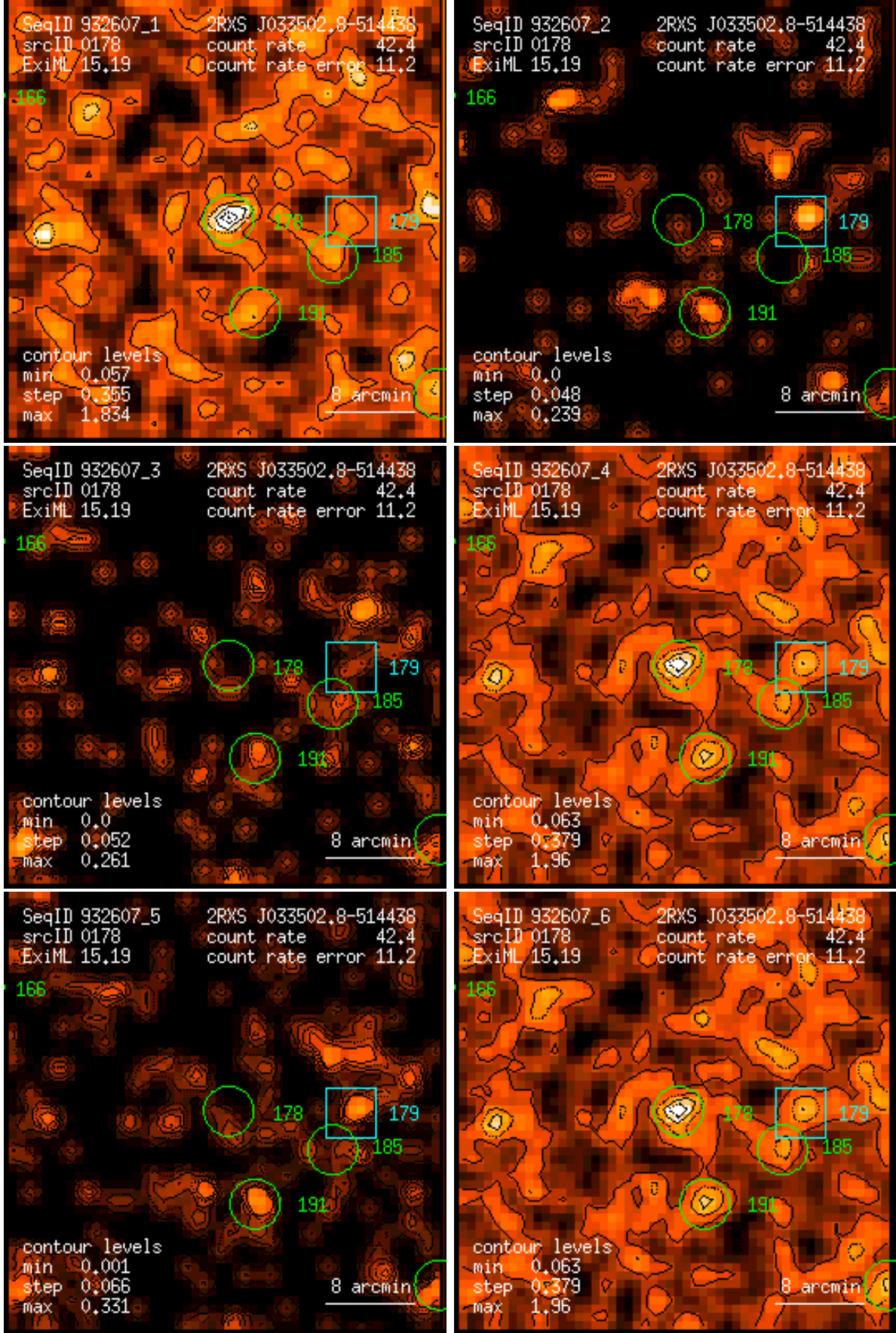
Figure 178: RASS 932607: detection 0178: band rate images, Gaussian filter: (1) PSPC channels 11 – 41, (2) 52 – 90, (3) 91 – 201, (4) 11 – 235, (5) 52 – 201, (6) 11 – 201. Broad band rates in counts/ks. Band rate contour levels in counts/ks/arcmin 2 .
