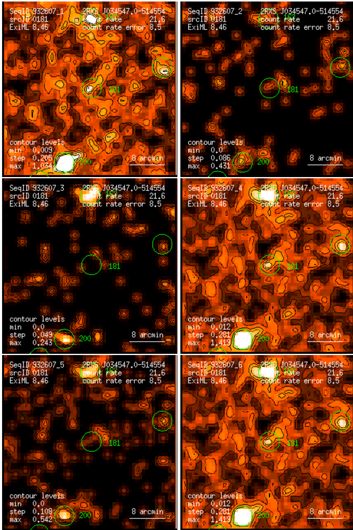
Figure 181: RASS 932607: detection 0181: band rate images, Gaussian filter: (1) PSPC channels 11 – 41, (2) 52 – 90, (3) 91 – 201, (4) 11 – 235, (5) 52 – 201, (6) 11 – 201. Broad band rates in counts/ks. Band rate contour levels in counts/ks/arcmin 2 .
