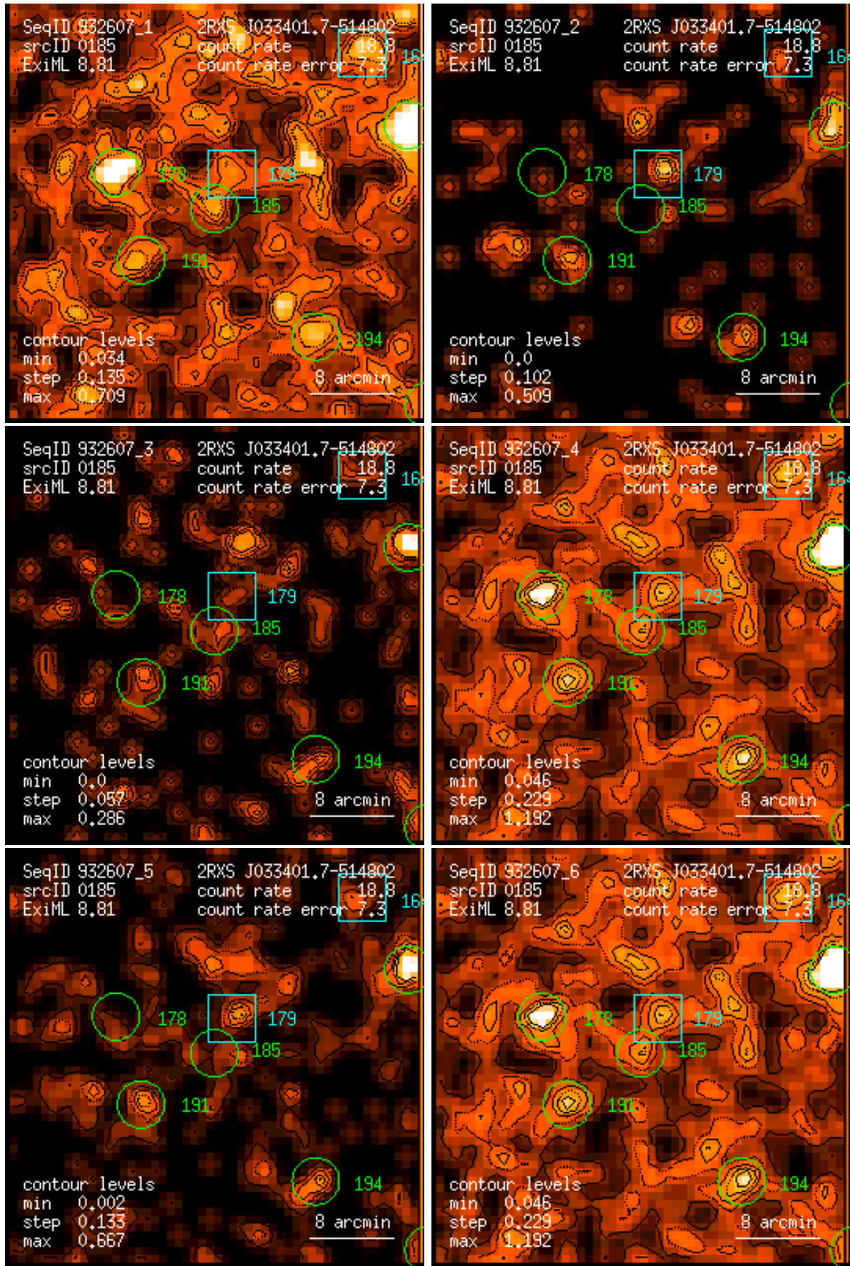
Figure 185: RASS 932607: detection 0185: band rate images, Gaussian filter: (1) PSPC channels 11 – 41, (2) 52 – 90, (3) 91 – 201, (4) 11 – 235, (5) 52 – 201, (6) 11 – 201. Broad band rates in counts/ks. Band rate contour levels in counts/ks/arcmin 2 .
