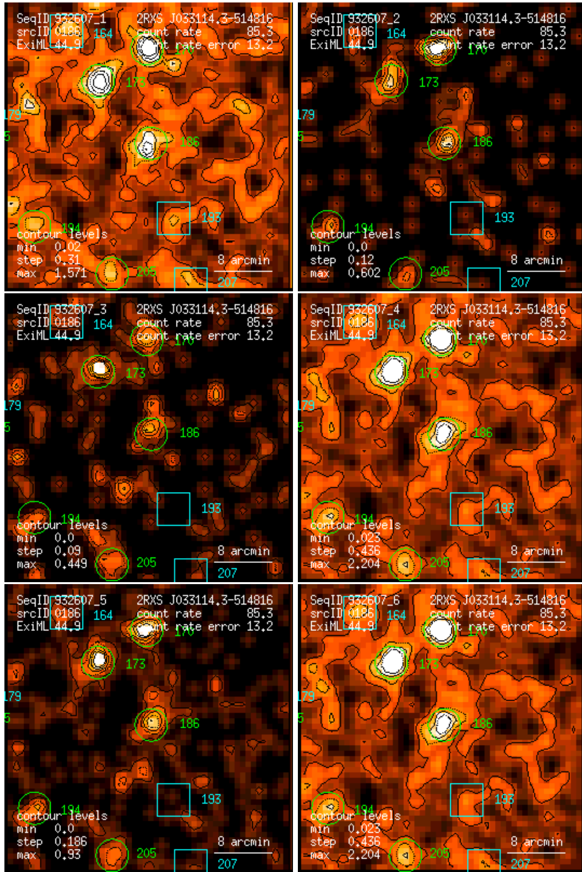
Figure 186: RASS 932607: detection 0186: band rate images, Gaussian filter: (1) PSPC channels 11 – 41, (2) 52 – 90, (3) 91 – 201, (4) 11 – 235, (5) 52 – 201, (6) 11 – 201. Broad band rates in counts/ks. Band rate contour levels in counts/ks/arcmin 2 .
