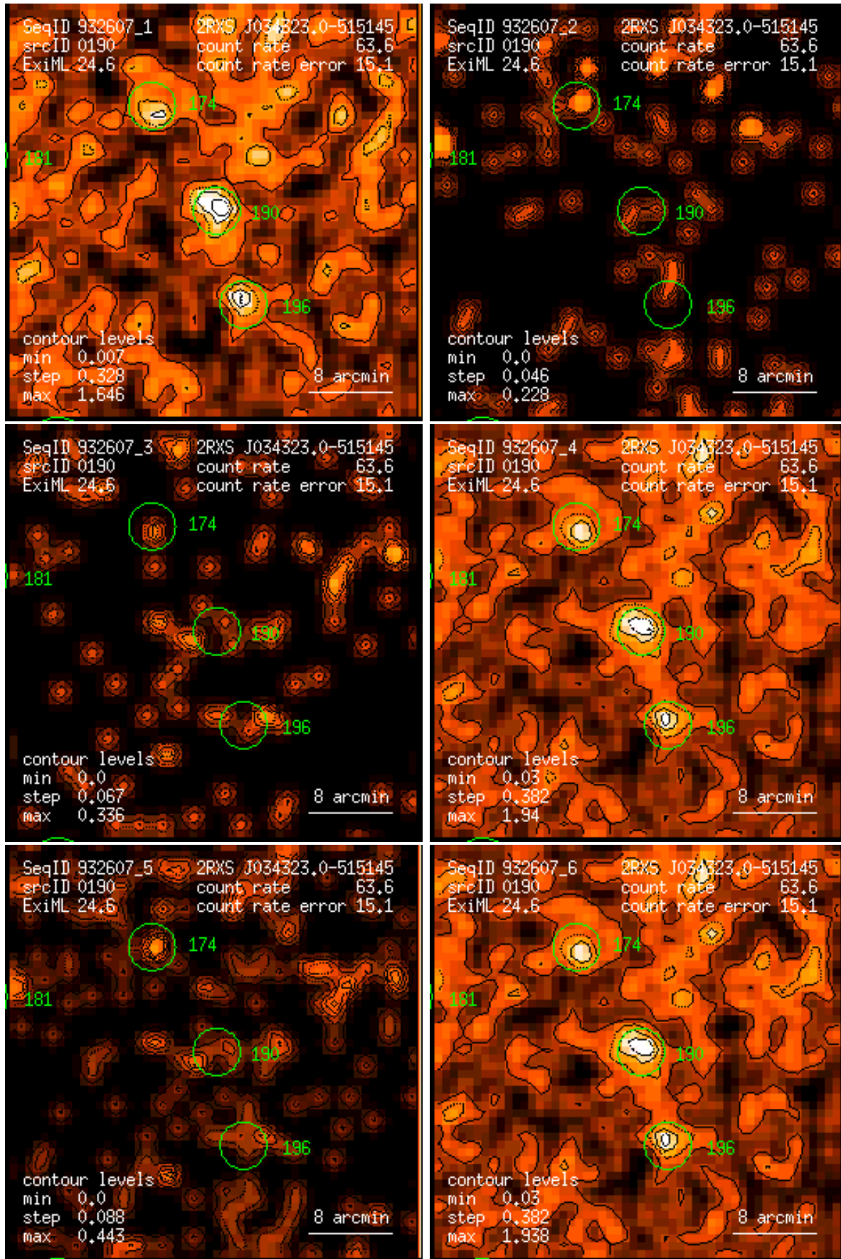
Figure 190: RASS 932607: detection 0190: band rate images, Gaussian filter: (1) PSPC channels 11 – 41, (2) 52 – 90, (3) 91 – 201, (4) 11 – 235, (5) 52 – 201, (6) 11 – 201. Broad band rates in counts/ks. Band rate contour levels in counts/ks/arcmin 2 .
