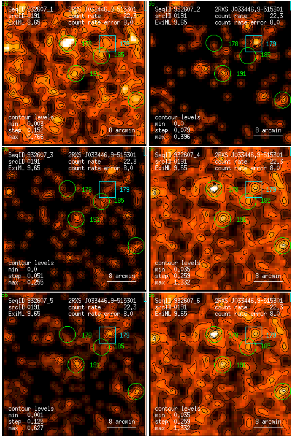
Figure 191: RASS 932607: detection 0191: band rate images, Gaussian filter: (1) PSPC channels 11 – 41, (2) 52 – 90, (3) 91 – 201, (4) 11 – 235, (5) 52 – 201, (6) 11 – 201. Broad band rates in counts/ks. Band rate contour levels in counts/ks/arcmin 2 .
