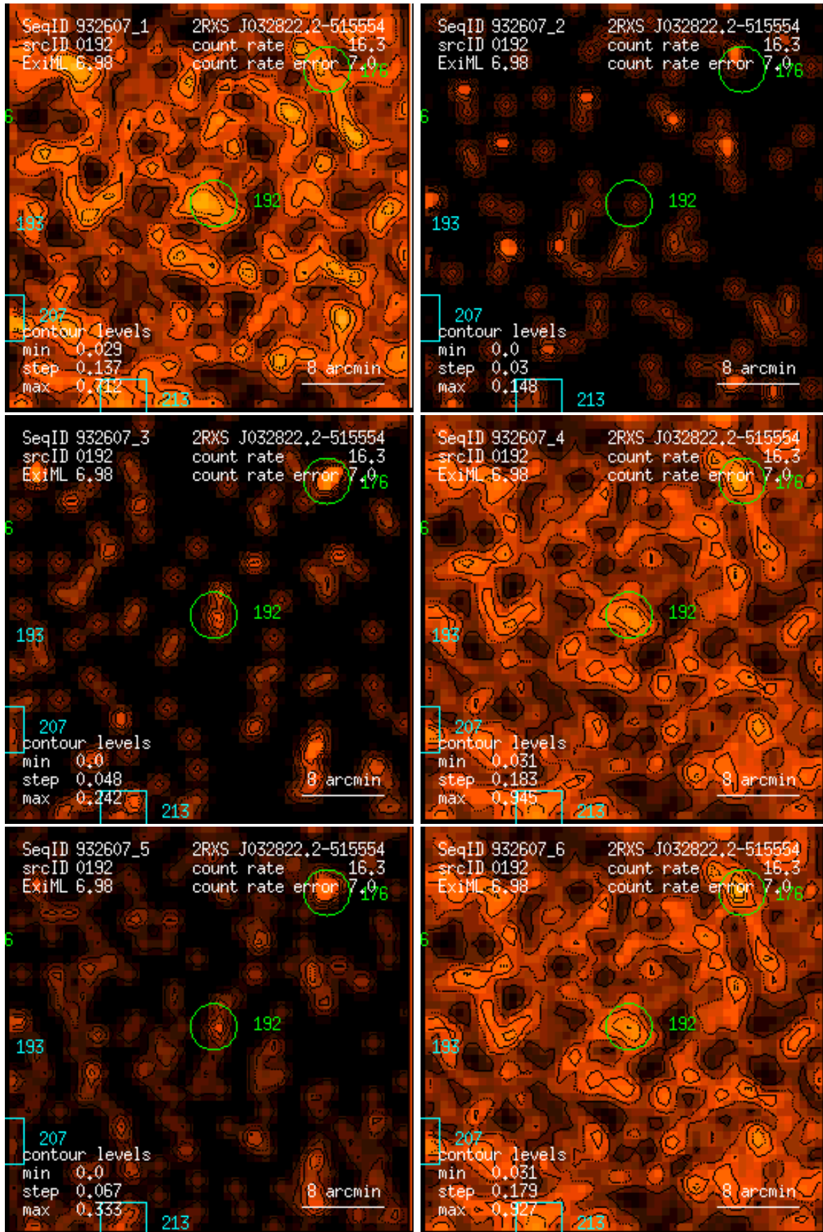
Figure 192: RASS 932607: detection 0192: band rate images, Gaussian filter: (1) PSPC channels 11 – 41, (2) 52 – 90, (3) 91 – 201, (4) 11 – 235, (5) 52 – 201, (6) 11 – 201. Broad band rates in counts/ks. Band rate contour levels in counts/ks/arcmin 2 .
