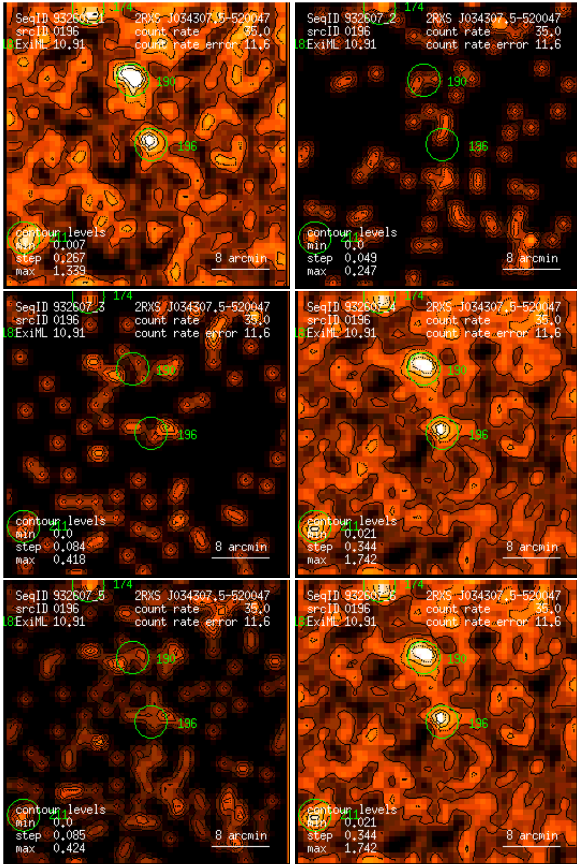
Figure 196: RASS 932607: detection 0196: band rate images, Gaussian filter: (1) PSPC channels 11 – 41, (2) 52 – 90, (3) 91 – 201, (4) 11 – 235, (5) 52 – 201, (6) 11 – 201. Broad band rates in counts/ks. Band rate contour levels in counts/ks/arcmin 2 .
