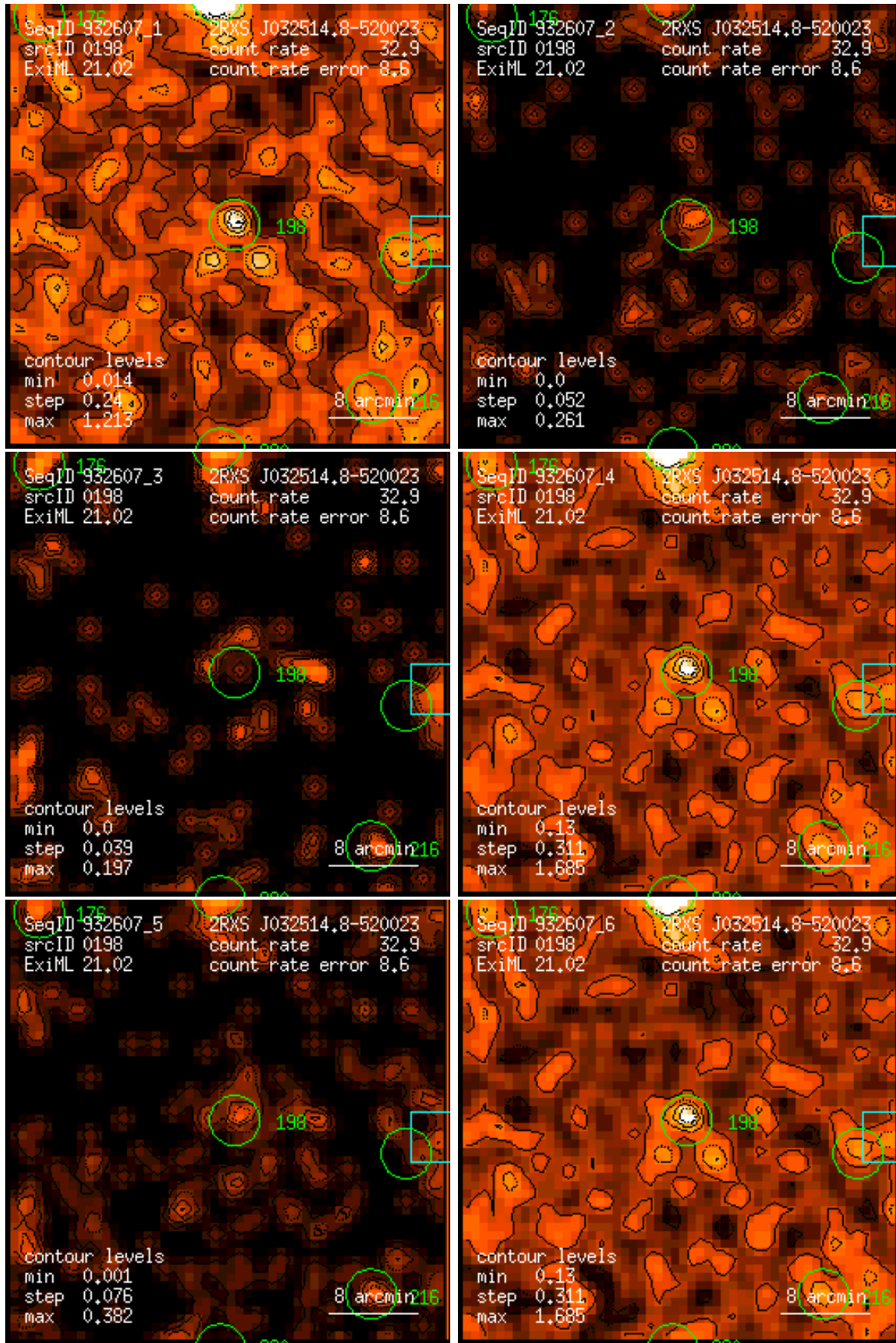
Figure 198: RASS 932607: detection 0198: band rate images, Gaussian filter: (1) PSPC channels 11 – 41, (2) 52 – 90, (3) 91 – 201, (4) 11 – 235, (5) 52 – 201, (6) 11 – 201. Broad band rates in counts/ks. Band rate contour levels in counts/ks/arcmin 2 .
