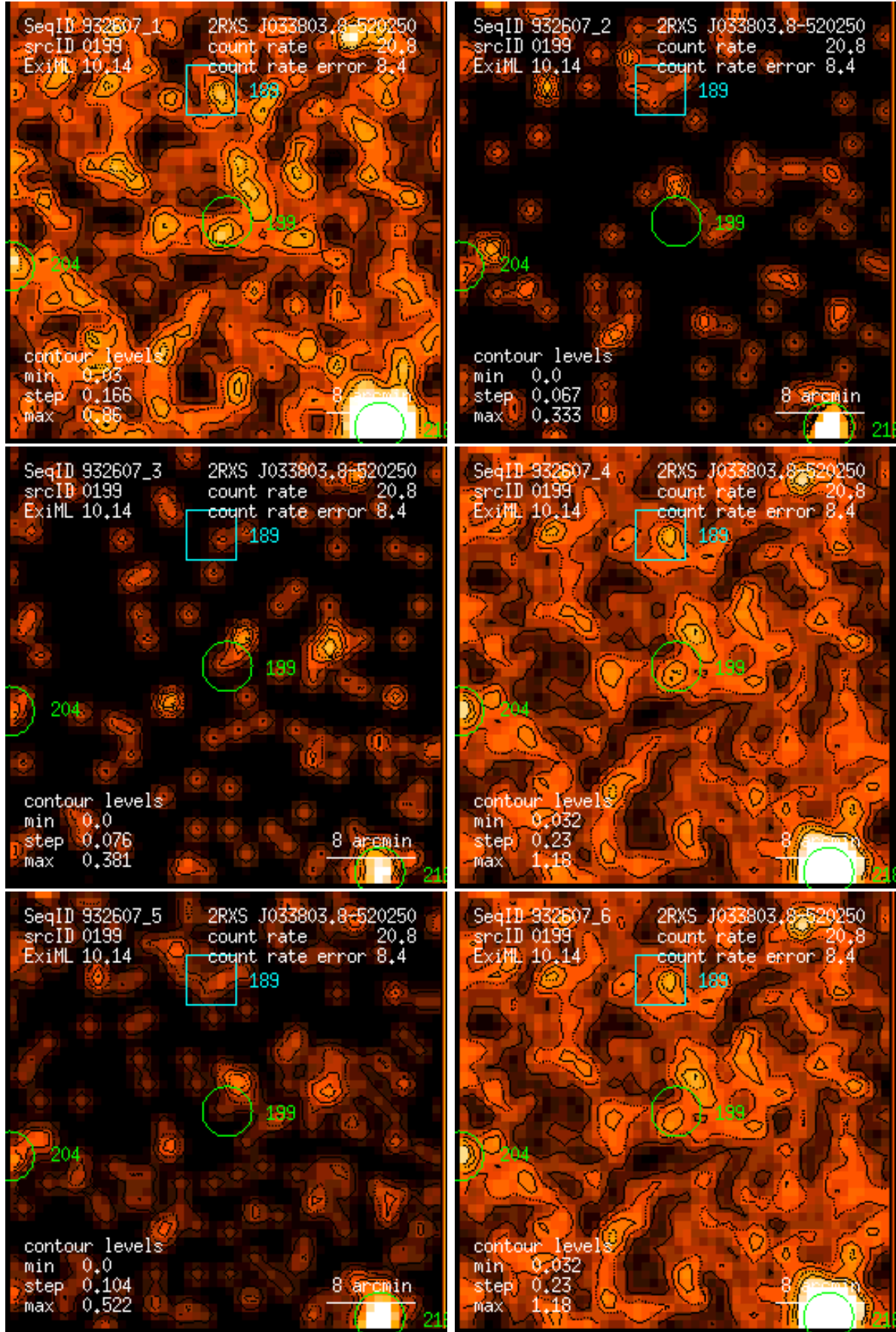
Figure 199: RASS 932607: detection 0199: band rate images, Gaussian filter: (1) PSPC channels 11 – 41, (2) 52 – 90, (3) 91 – 201, (4) 11 – 235, (5) 52 – 201, (6) 11 – 201. Broad band rates in counts/ks. Band rate contour levels in counts/ks/arcmin 2 .
