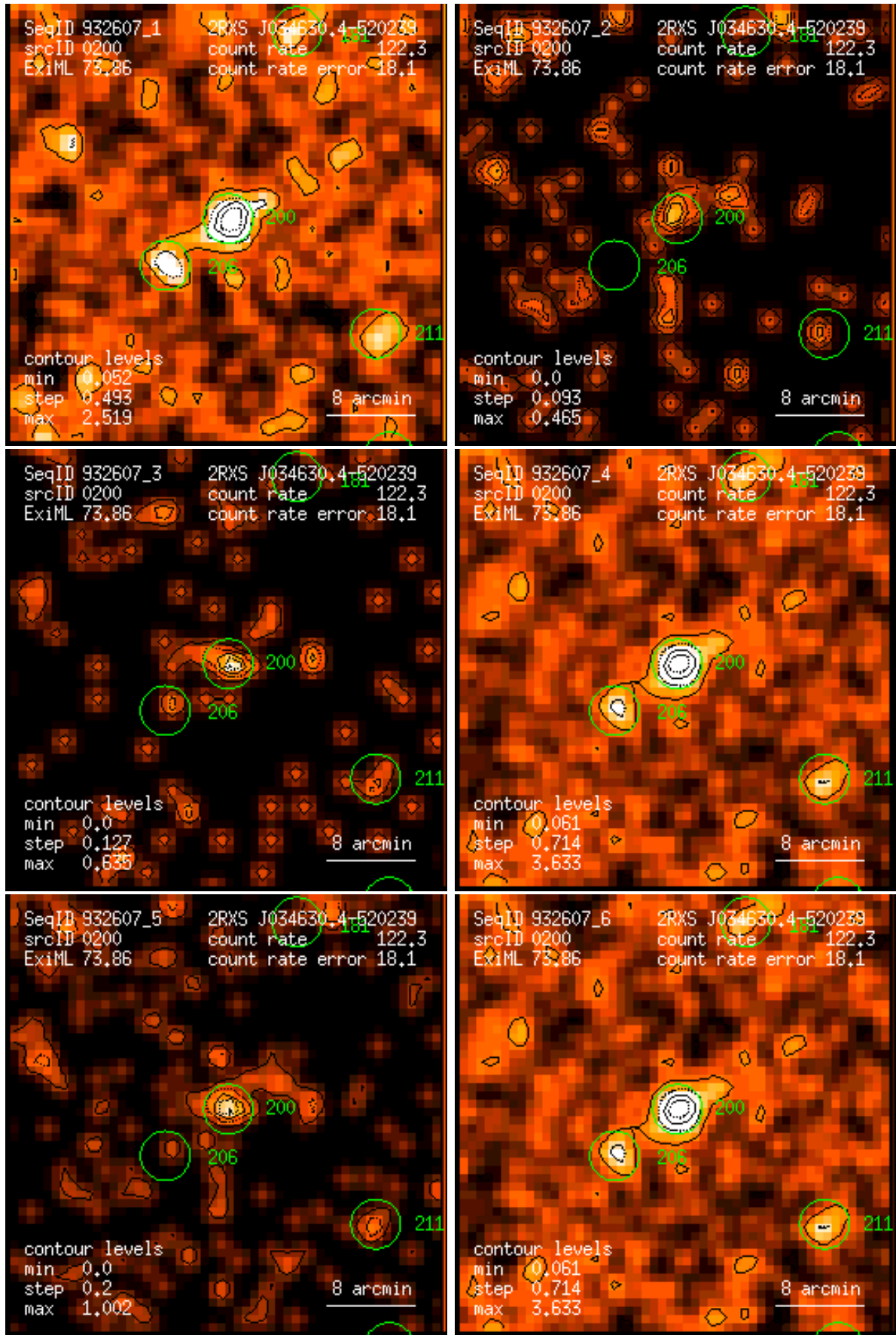
Figure 200: RASS 932607: detection 0200: band rate images, Gaussian filter: (1) PSPC channels 11 – 41, (2) 52 – 90, (3) 91 – 201, (4) 11 – 235, (5) 52 – 201, (6) 11 – 201. Broad band rates in counts/ks. Band rate contour levels in counts/ks/arcmin 2 .
