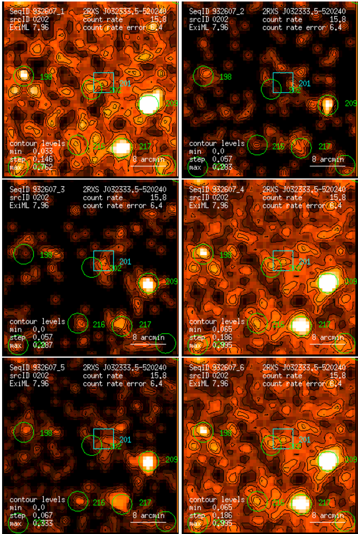
Figure 202: RASS 932607: detection 0202: band rate images, Gaussian filter: (1) PSPC channels 11 – 41, (2) 52 – 90, (3) 91 – 201, (4) 11 – 235, (5) 52 – 201, (6) 11 – 201. Broad band rates in counts/ks. Band rate contour levels in counts/ks/arcmin 2 .
