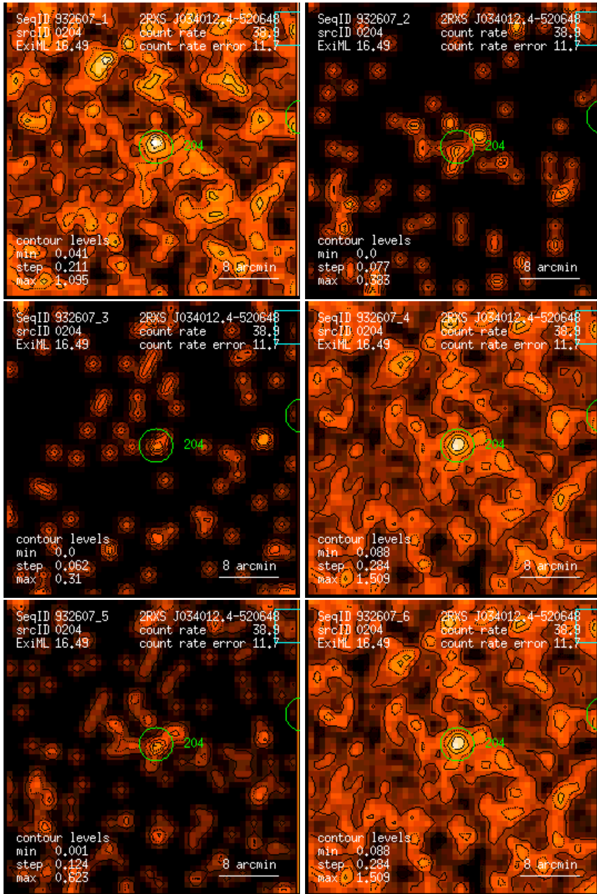
Figure 204: RASS 932607: detection 0204: band rate images, Gaussian filter: (1) PSPC channels 11 – 41, (2) 52 – 90, (3) 91 – 201, (4) 11 – 235, (5) 52 – 201, (6) 11 – 201. Broad band rates in counts/ks. Band rate contour levels in counts/ks/arcmin 2 .
