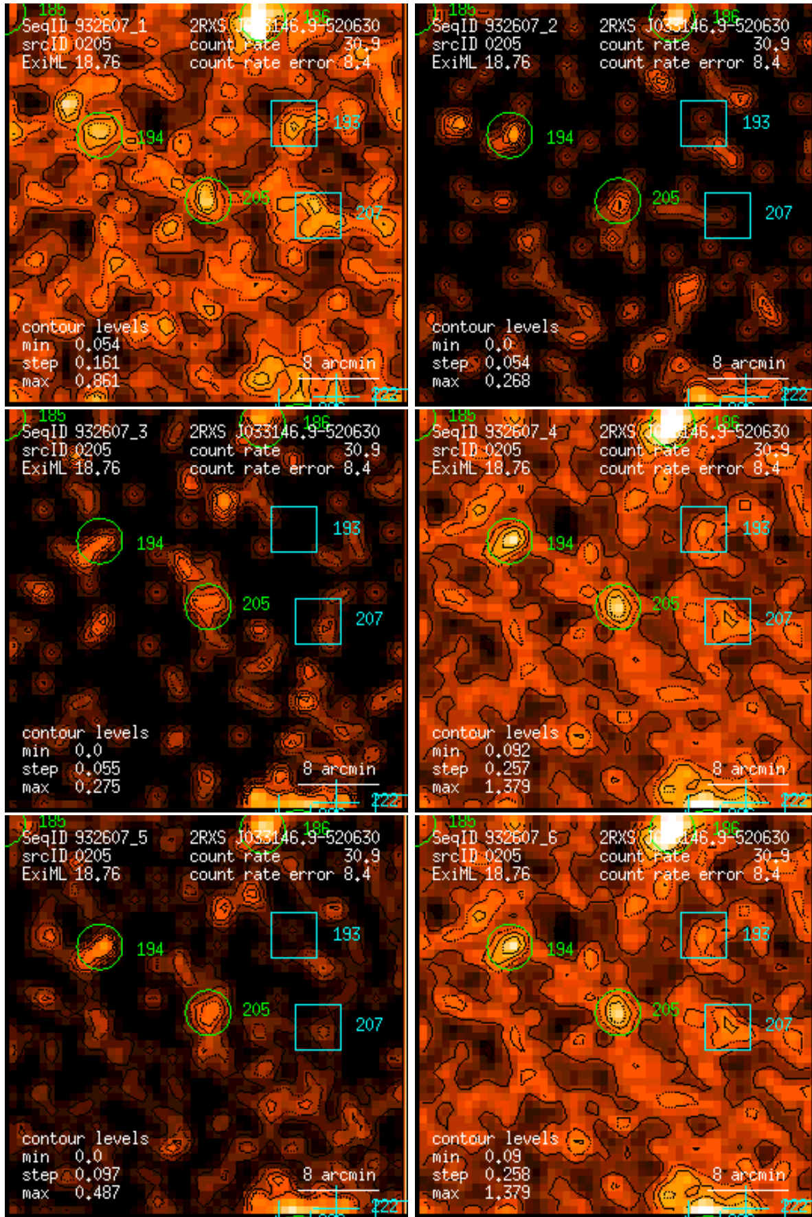
Figure 205: RASS 932607: detection 0205: band rate images, Gaussian filter: (1) PSPC channels 11 – 41, (2) 52 – 90, (3) 91 – 201, (4) 11 – 235, (5) 52 – 201, (6) 11 – 201. Broad band rates in counts/ks. Band rate contour levels in counts/ks/arcmin 2 .
