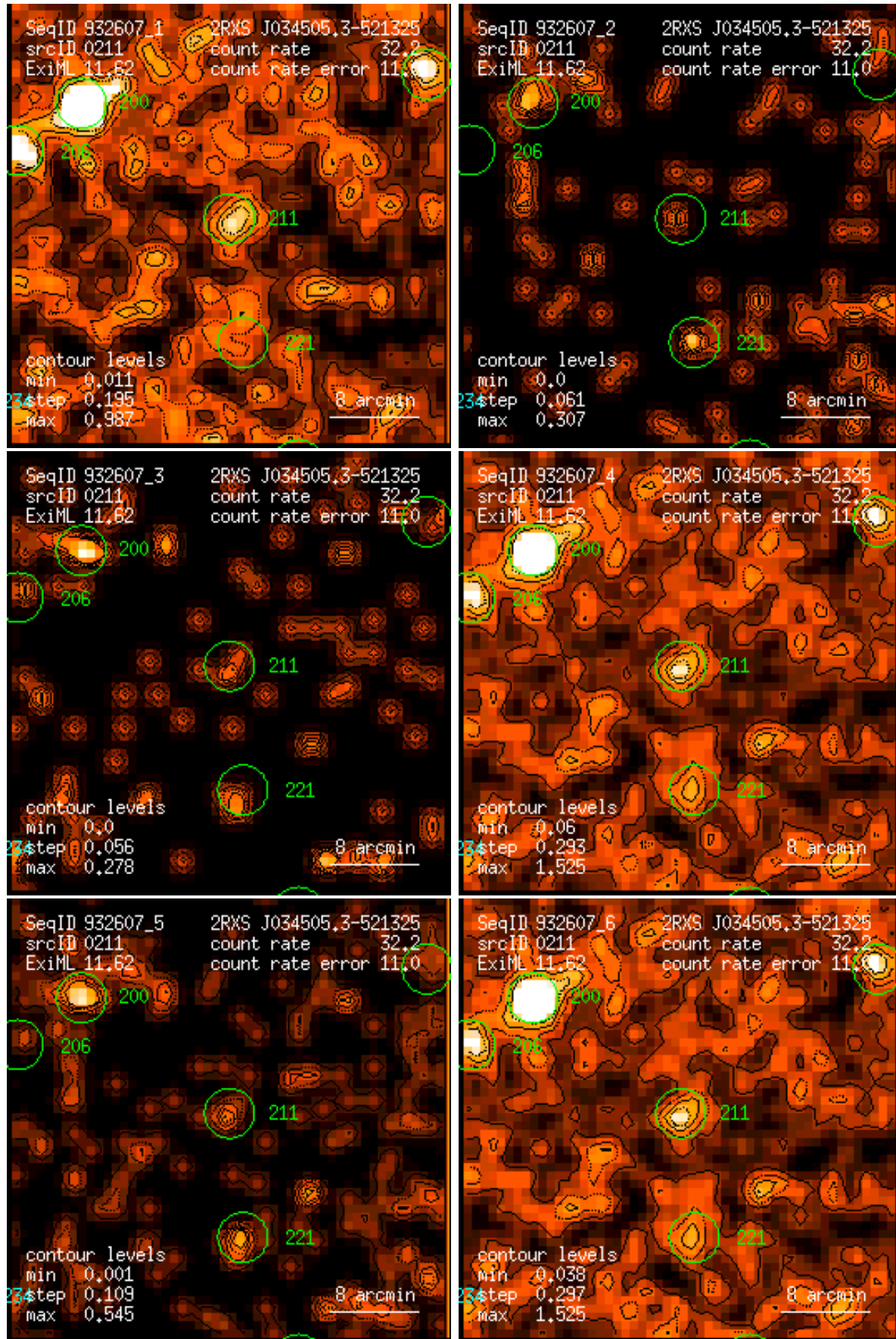
Figure 211: RASS 932607: detection 0211: band rate images, Gaussian filter: (1) PSPC channels 11 – 41, (2) 52 – 90, (3) 91 – 201, (4) 11 – 235, (5) 52 – 201, (6) 11 – 201. Broad band rates in counts/ks. Band rate contour levels in counts/ks/arcmin 2 .
